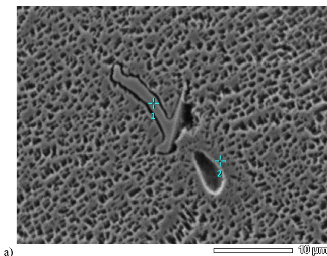
a) The Cr and Mo- enriched carbide particles, b) The chemical composition of Cr and Mo- enriched carbide particles
