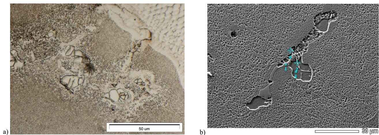
Fig. 5. The microstructure of the IN 713C with the ( \gamma + \gamma' ) eutectic islands: a) LM, b) SEM
