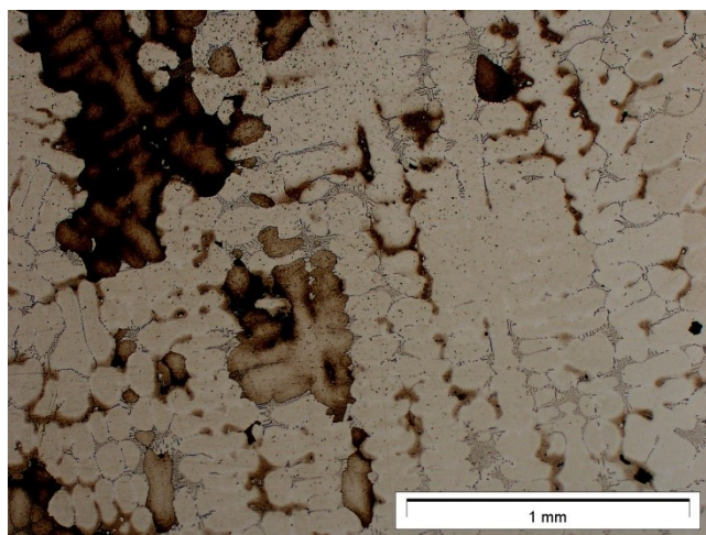
Fig. 1. Microstructure of IN 713C alloy in the as-cast condition; LM
