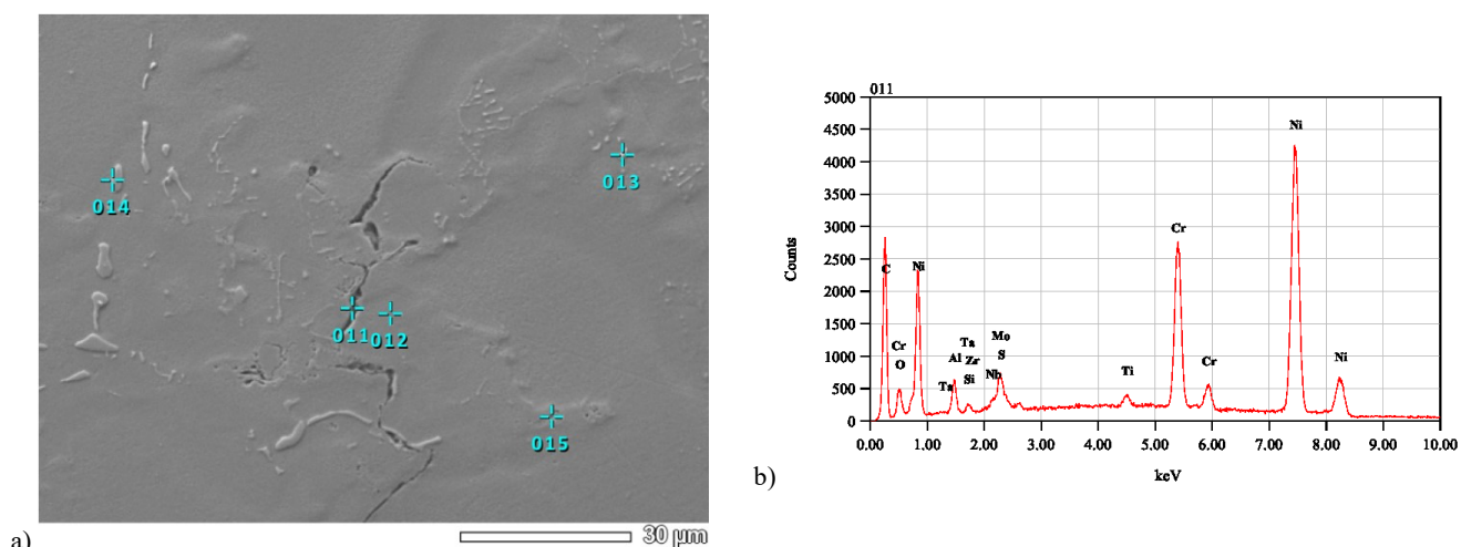
Fig. 6. a) The crack identified in the structure of the pad weld, b) The chemical composition of the crack
