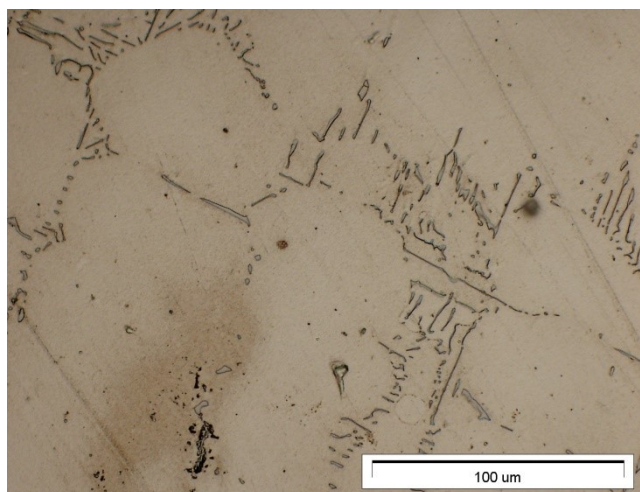
Fig. 2. Structure of IN 713C alloy with „Chinese scripts”
