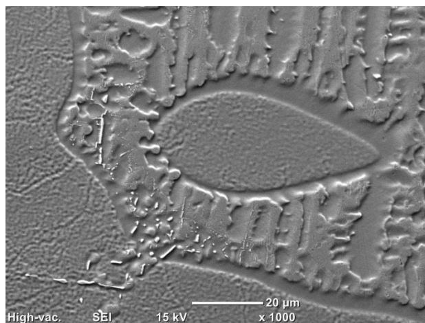
Fig. 4. The fusion line with the PFZ area
