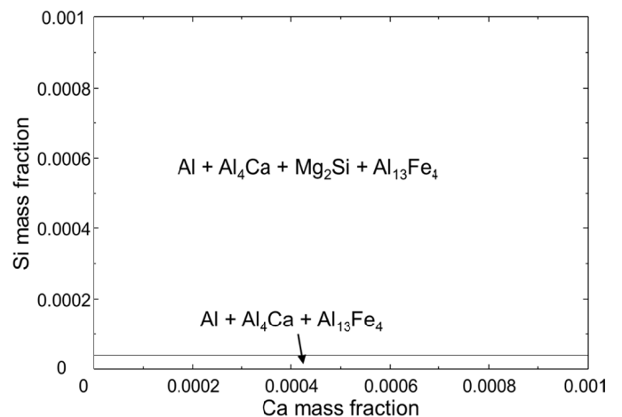
Fig. 3. Phase diagram plotted for Si versus Ca mass fractions at 490^\circ\text{C} calculated by FactSage 7.3 . The contents of Mg and Fe are fixed at those mentioned in the section of Experimental
