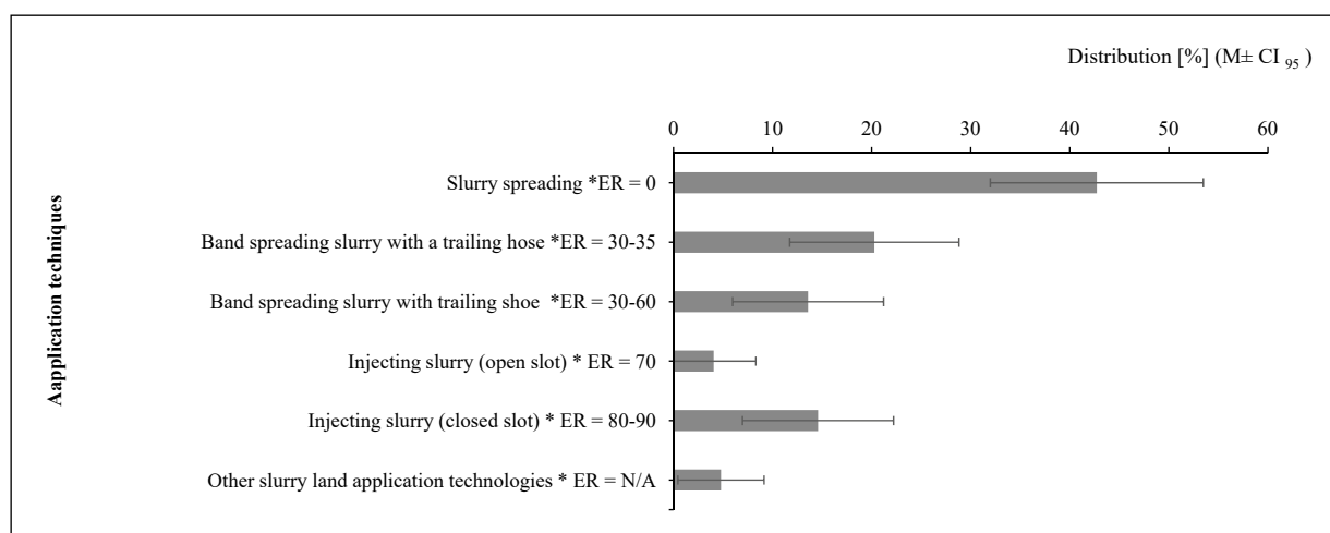
Fig. 2. Ammonia emission abatement measures for pig slurry storage
