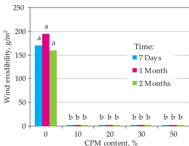
Fig. 3. Means of the wind erodibility index after various times depending on CPM content in solution used for treatment
