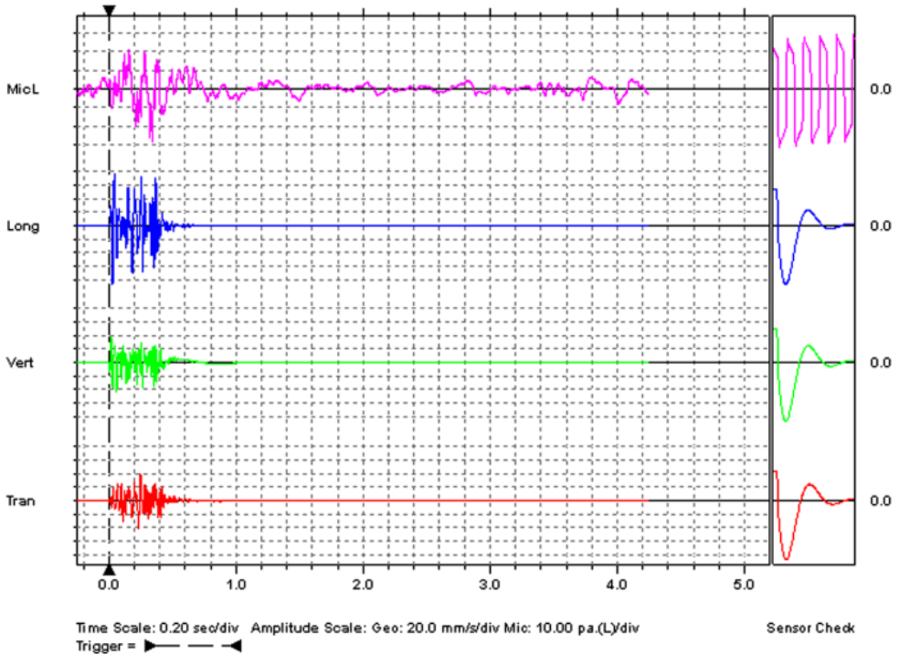
Fig. 6. Measured vibration and noise levels in the drill cuttings stemming test at Asagi Caglayan basalt quarry
