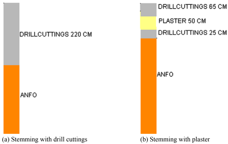
Fig. 2. Blast hole stemming at Asagi Caglayan basalt quarry
