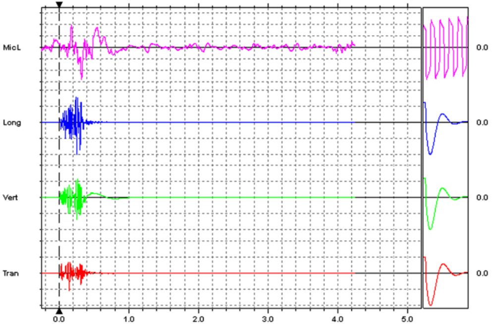
Fig. 7. Measured vibration and noise levels in the plaster stemming test at Asagi Caglayan
