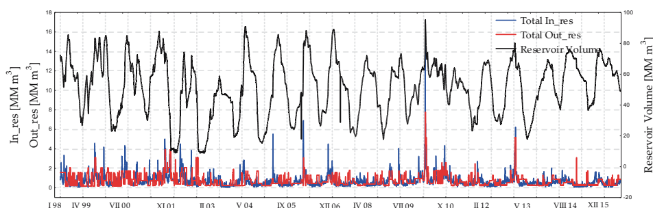
Fig. 2. Daily values of inflow and outflow to and from the Turawa reservoir and the reservoir capacity in 1998–2016
