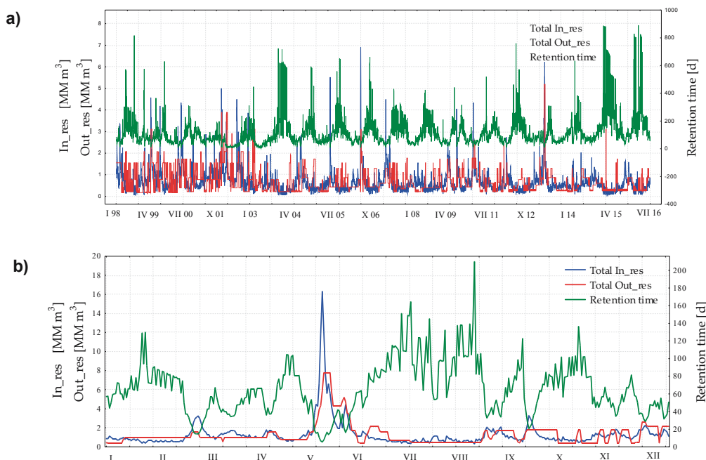
Fig. 3. The amount of water flowing into the Turawa reservoir (In_res) and the amount of water flowing out of it (Out_res) compared to the variability of retention time (monthly values): a) in 1998–2009 and 2011–2016, b) in 2010
