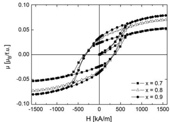
Fig. 4. Room-temperature hysteresis loops of (\text{BiFeO}_3)_x\text{-(BaTiO}_3)_{1-x} solid solutions sintered at 1103 K.
