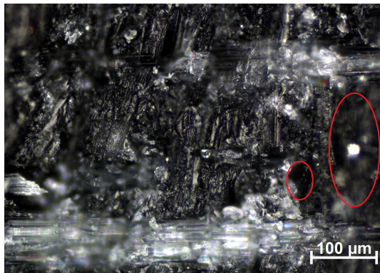
Fig. 2. A photograph of the composite structure with a 10% glass polyester waste content ( \leq 1.2 mm grain size), with defects marked, taken with an optical microscope.
