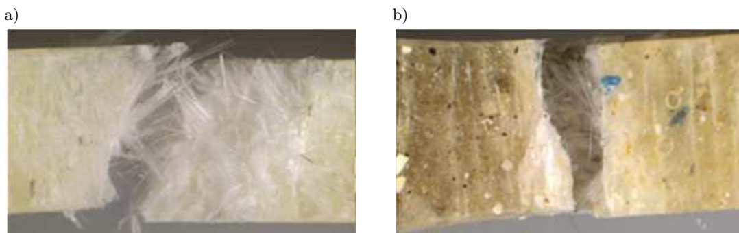
Fig. 10. Samples after static tensile testing: a) sample without recycle, b) sample with 10% recycle content.
