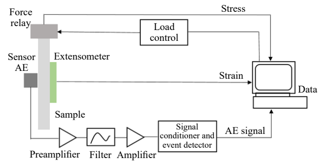
Fig. 4. Diagram of the measuring station.
