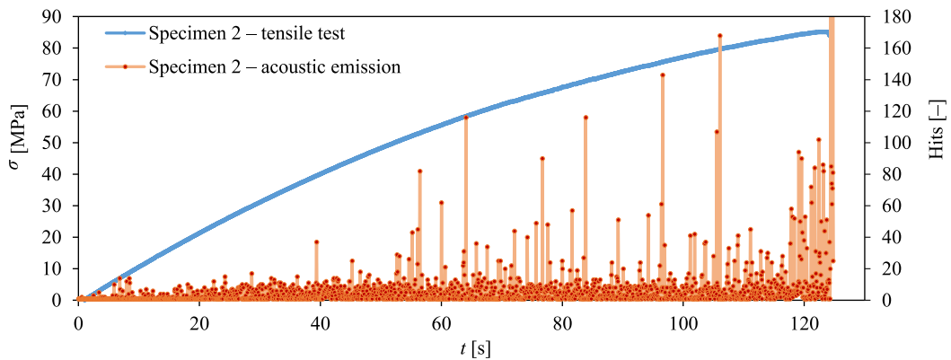
Fig. 7. Graph of stress and number of AE hits as a function of time for a selected sample with 10% recycle content.
