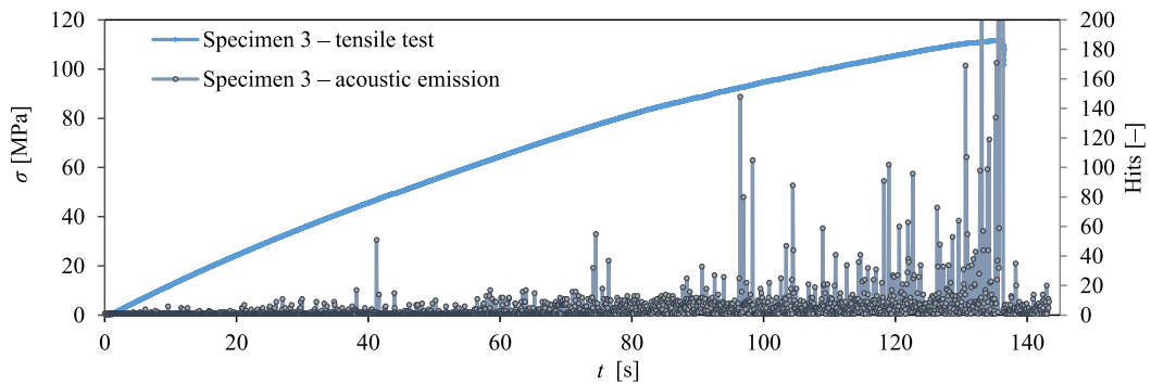
Fig. 6. Graph of stress and number of AE hits, as a function of time for a selected sample without recycle.
