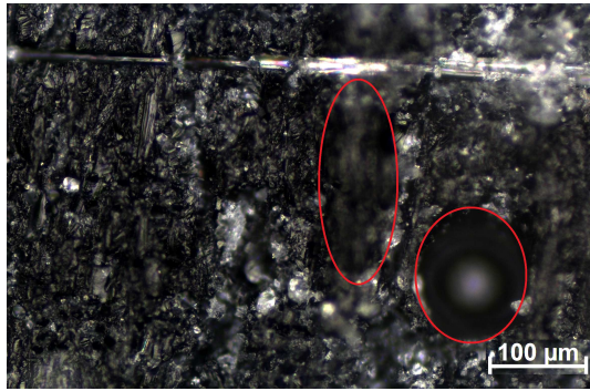
Fig. 1. A photograph of the composite structure without any glass polyester waste content, with defects marked, taken with an optical microscope.
