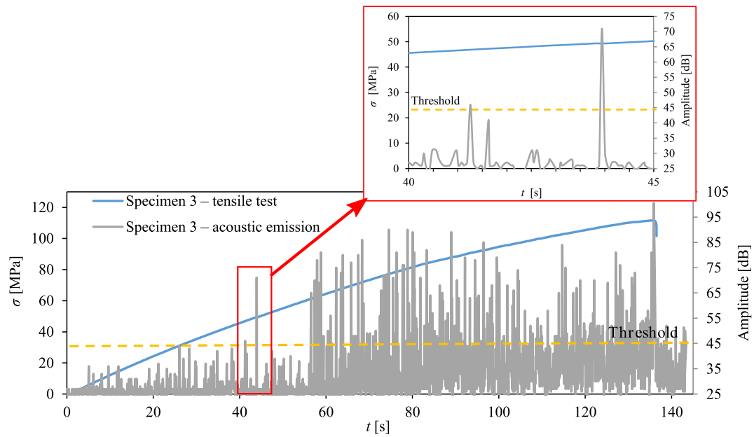
Fig. 8. Graph of stress and amplitude of acoustic emission signals as a function of time for a sample without recycle.
