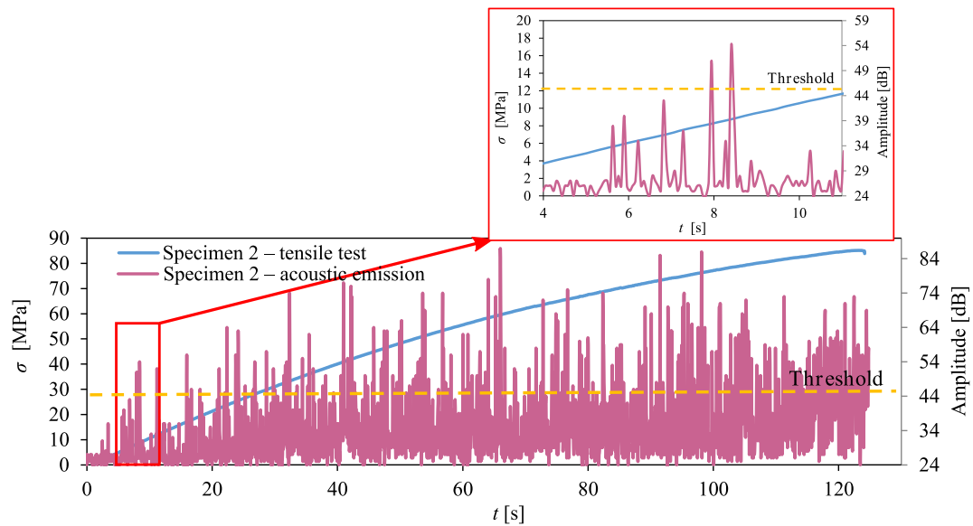
Fig. 9. Graph of stress and amplitude of acoustic emission signals as a function of time for a sample with 10% polyester-glass recycle content.
