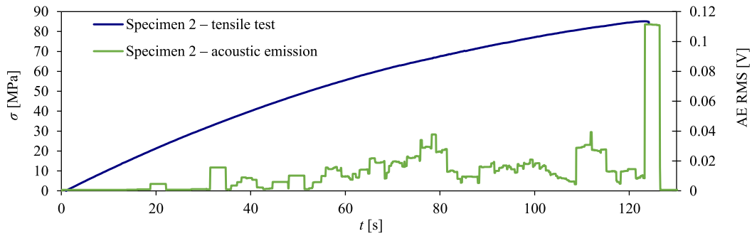
Fig. 12. Stress and RMS graph as a function of time for a sample with 10% polyester-glass recycle content.
