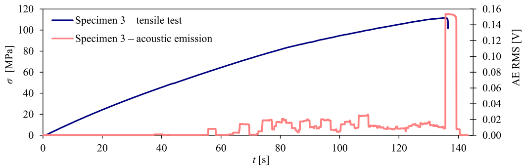
Fig. 11. Stress and RMS graph as a function of time for a sample without recycle.
