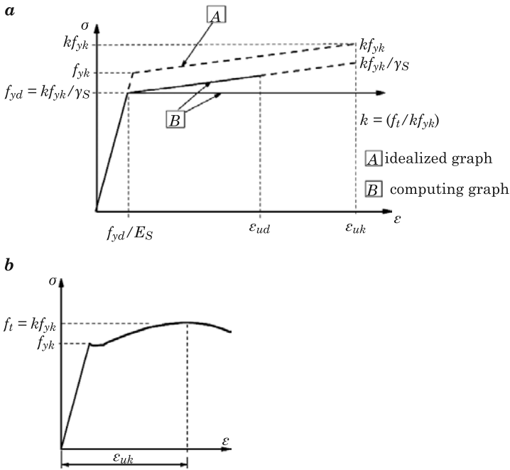
Fig. 7. Stress-strain graph of reinforcing steel, model in program (computing graph) (a), Stress-strain graph of a typical reinforcing steel (b)
