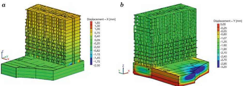
Fig. 12. Maximum horizontal displacement of construction in direction X (a), maximum horizontal displacement of construction in direction Y (b)
