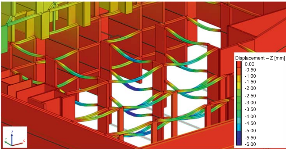
Fig. 11. Maximum vertical displacement of lintels and substrings
