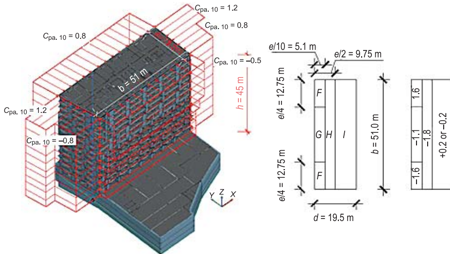
Fig. 8. Pressure peaks of wind speed, together with the distribution of external pressure c_{pe,10} Source: own elaboration.
