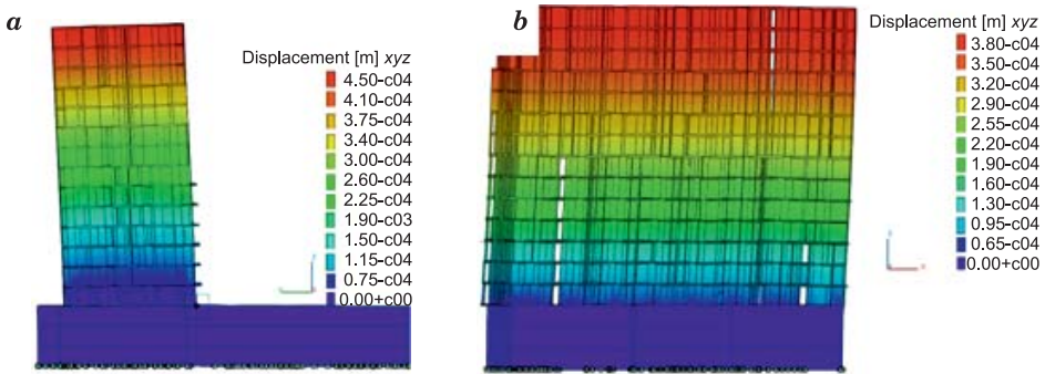
Fig. 9. First form of vibration model in the plane zy, for 2.71 Hz (a), second form of vibration model in the plane zx, for 3.01 Hz (b)
