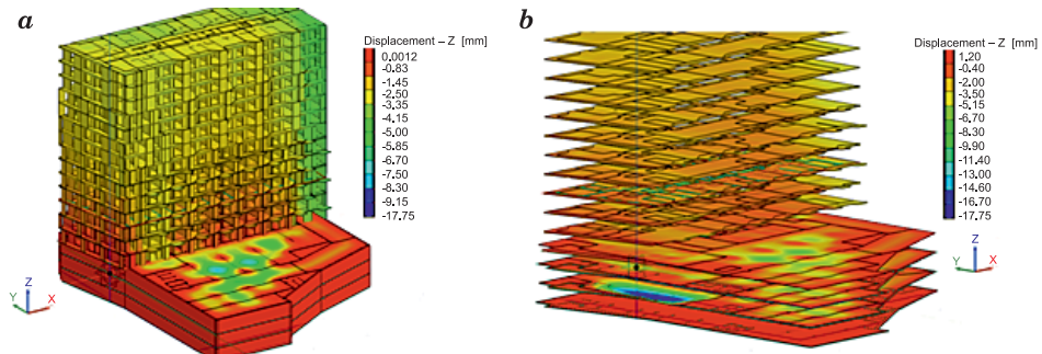
Fig. 10. Maximum vertical displacement building (a), maximum vertical displacement of slabs (b)
