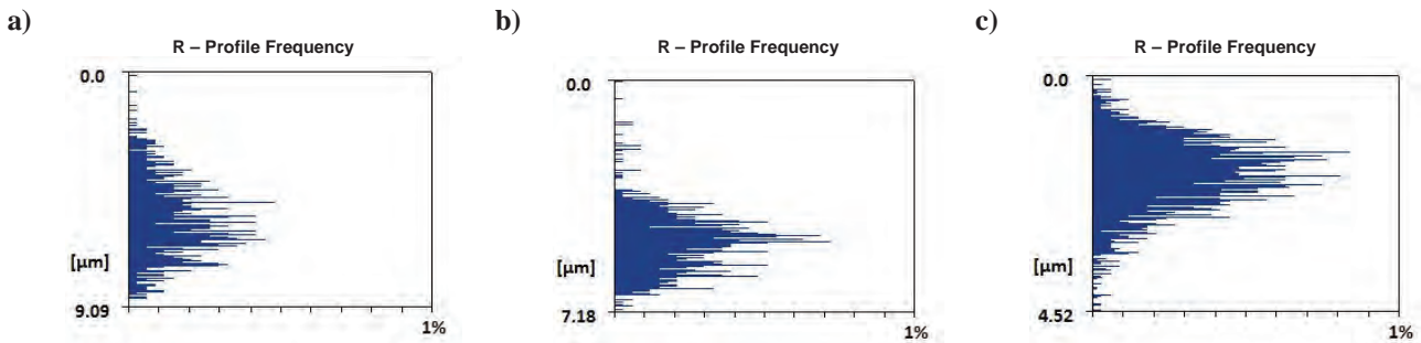
Fig. 6. The skewness for intermetallic coatings \text{Ni}_3\text{Al} for cutting inserts: a) square SNGA 120408 S01030A CB7015 ( R_{sk} = 0.407 \mu\text{m} ) and b) trigon WNMG 080408 S01030A CB7015 ( R_{sk} = 0.909 \mu\text{m} ) and c) trigon WNMG 080408 - KF with GC3215 ( R_{sk} = -0.423 \mu\text{m} )
