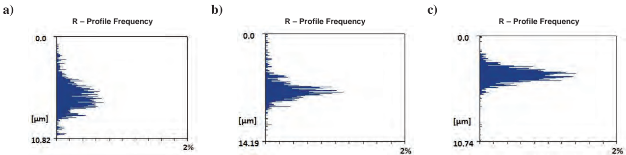
Fig. 5. The skewness for intermetallic coatings \text{NiAl} for cutting inserts: a) square SNGA 120408 S01030A CB7015 ( R_{sk} = 0.415 \mu\text{m} ) and b) trigon WNMG 080408 S01030A CB7015 ( R_{sk} = 1.044 \mu\text{m} ) and c) trigon WNMG 080408 - KF GC3215 ( R_{sk} = -0.537 \mu\text{m} )
