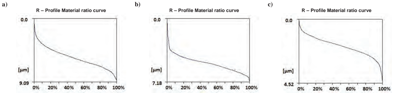
Fig. 4. The material ratio curve surface roughness intermetallic coatings \text{Ni}_3\text{Al} for cutting inserts: a) square SNGA 120408 S01030A CB7015 ( R_a = 1.18 \mu\text{m} ) and b) trigon WNMG 080408 S01030A CB7015 ( R_a = 0.71 \mu\text{m} ) and c) trigon WNMG 080408 - KF with GC3215 ( R_a = 0.55 \mu\text{m} )
