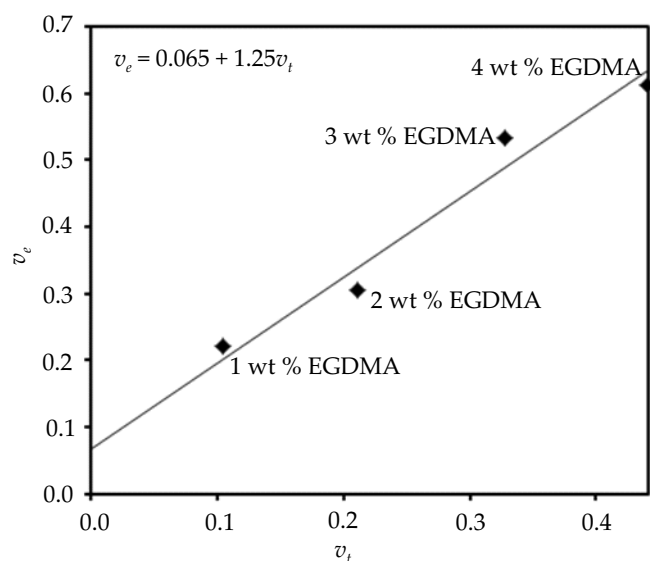
Fig. 6. Dependence of measured effective crosslink density ( v_e ) on theoretical crosslink density ( v_t ) for the gels at different amounts of EGDMA
