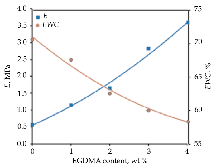
Fig. 5. The dependence of EWC and Young's modulus (E) for NVP90/TMSPM10 hydrogels system on the concentration of EGDMA
