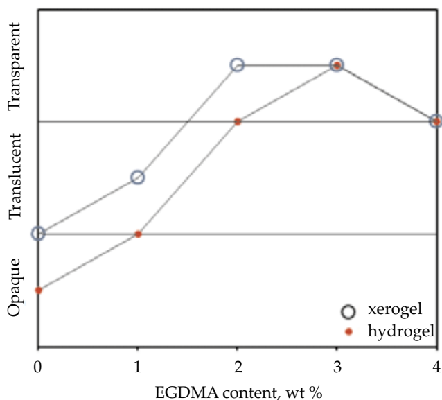
Fig. 4. Optical homogeneity of NVP90/TMSPM10 xerogels and hydrogels with various amount of EGDMA
