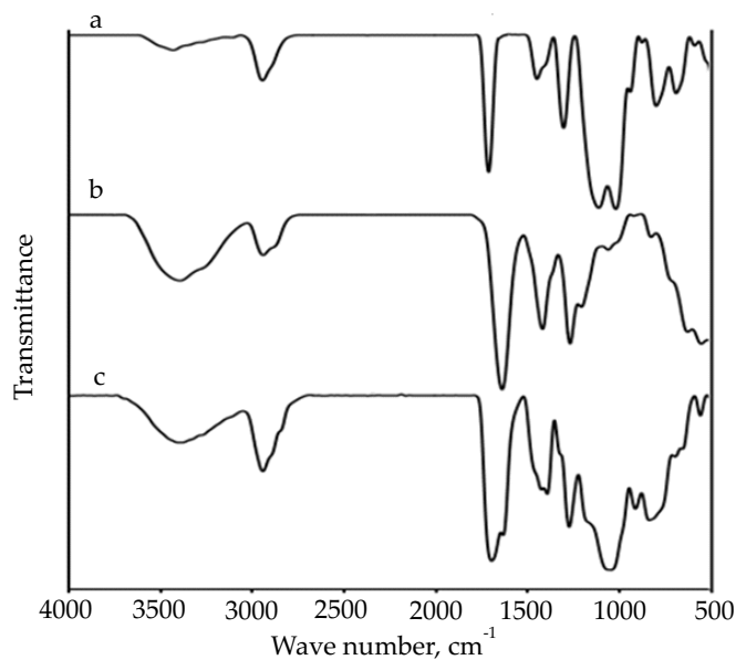
Fig. 1. FT-IR spectra of: a – PTMSPM, b – PNVP, c – NVP-co-TMSPM
