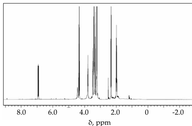
Fig. 2. ^1\text{H-NMR} spectrum of NVP-co-TMSPM copolymer
