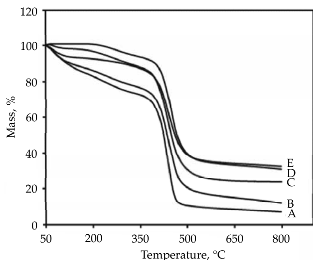
Fig. 7. TGA thermograms for NVP90/TMSPM10 xerogels containing: A – 0.0, B – 1.0, C – 2.0, D – 3.0, E – 4.0 wt % EGDMA
