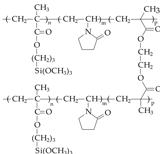
Scheme A. Schematic illustration of the structure of NVP-co-TMSPM crosslinked via EGDMA
