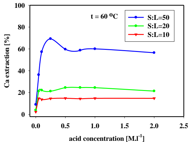
Fig. 9. Calcium extraction depending on L:S ratio
