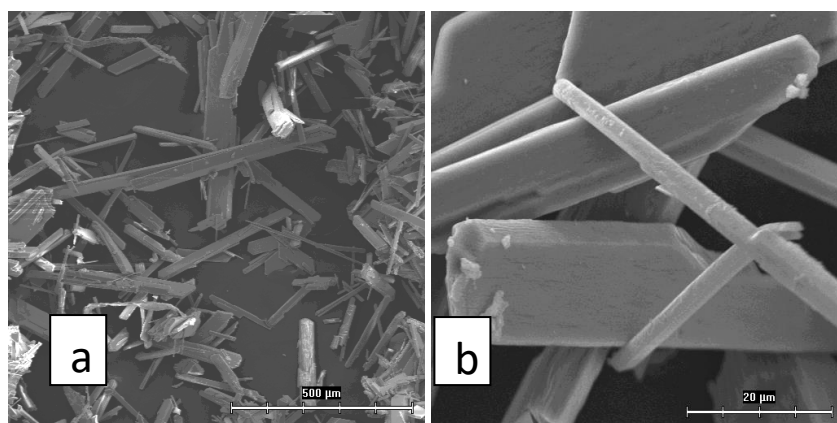
Fig. 13. Morphological observation on white precipitate
