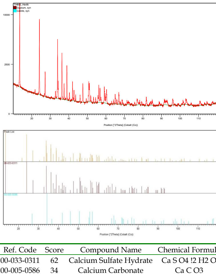
Fig. 12. X-Ray diffraction pattern of white precipitate
