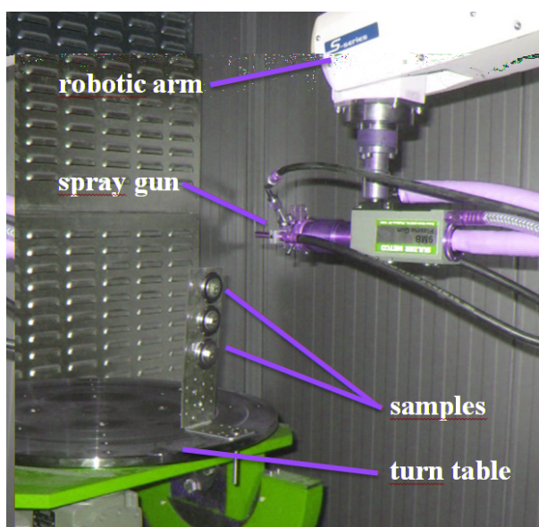
Fig. 3. Aspect of the plasma spray process
