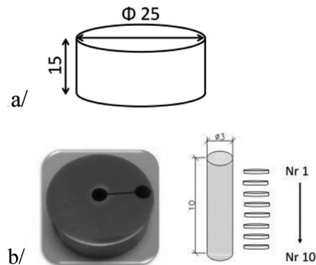
Fig. 1. The scheme of: a) specimen dimensions in millimeters and b) sites where the material for tests was sampled from
