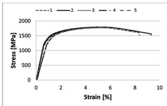
Fig. 4. Diagram of the interdependence between the stress and strain for specimens from 100CrMnSi6-4 steel with a nanobainitic structure
