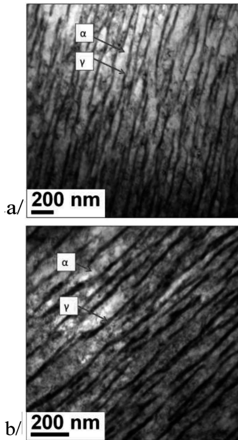
Fig. 2. The nanobainitic structure (light phase – bainitic ferrite, dark phase – retained austenite) obtained in the processes with identical treatment parameters in two various devices: a) in dilatometer, b) in industrial furnace
