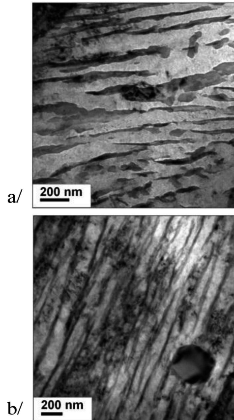
Fig. 3. a) Sample carbide-free structure (that is the structure with the bainitic ferrite or austenite plate width above 100nm), b) carbide found in the nanobainitic structure formed in the industrial furnace process
