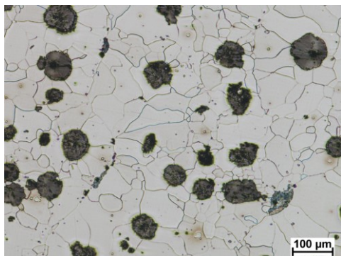
Fig. 3. Ductile cast iron, magnification 100x
