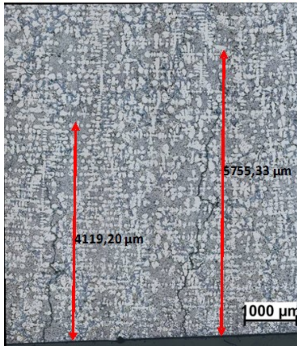
Fig. 8. Macroscopic view of samples after cycles of test and view of microstructure with marked length of cracks- Ductile cast iron
