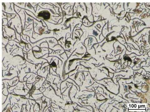
Fig. 5. Grey cast iron, magnification 100x
