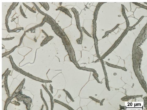
Fig. 6. Grey cast iron, magnification 500x
