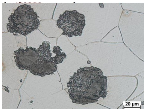
Fig. 4. Ductile cast iron, magnification 500x
