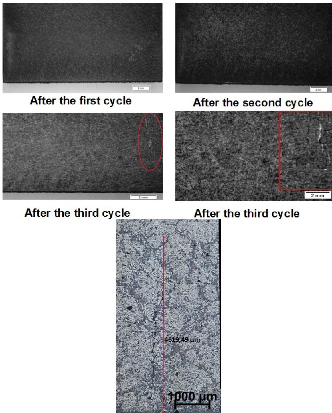
Fig. 9. Macroscopic view of samples after cycles of test and view of microstructure with marked length of cracks- Grey cast iron
