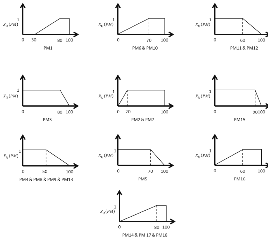
Fig. 7. The schematic figure of PMs fuzzy number.
