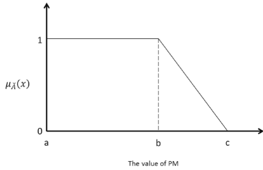
Fig. 3. The right trapezoidal fuzzy number for PM evaluation.
