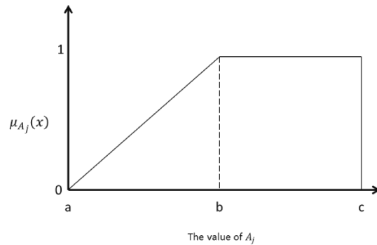
Fig. 5. Left trapezoidal Fuzzy number for the A j .
