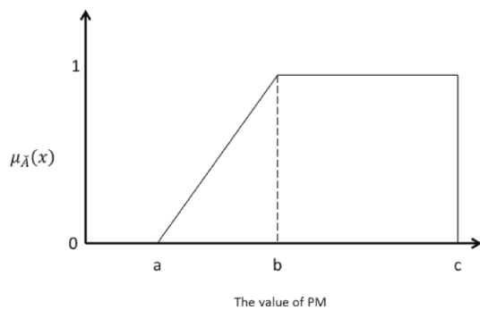
Fig. 4. The left trapezoidal fuzzy number for PM evaluation.
