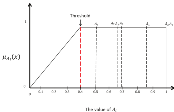
Fig. 8. The fuzzy number of A_i .
