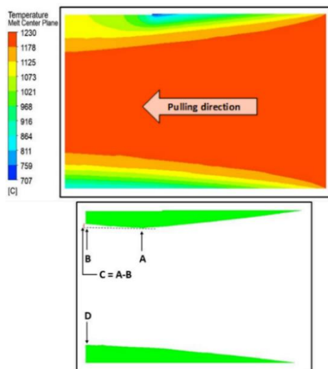
Fig. 5. 3D representation of solidified shell at the center (Top);
