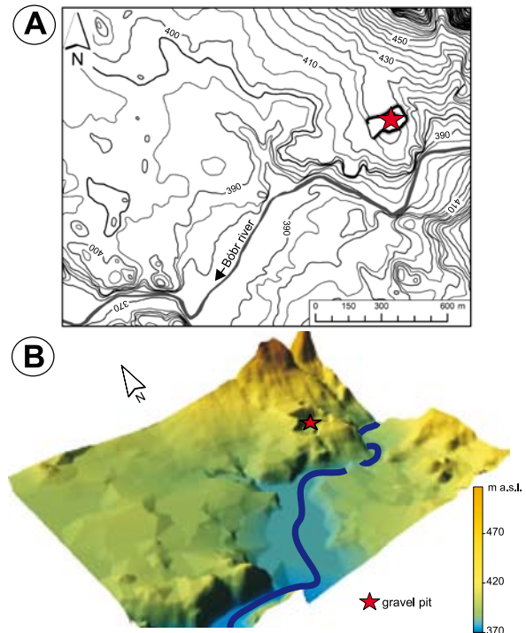
Fig. 2. A - Hypsometric map of the area around the Janowice Wielkie gravel pit; B - Shaded perspective images of the terrain's surface.
