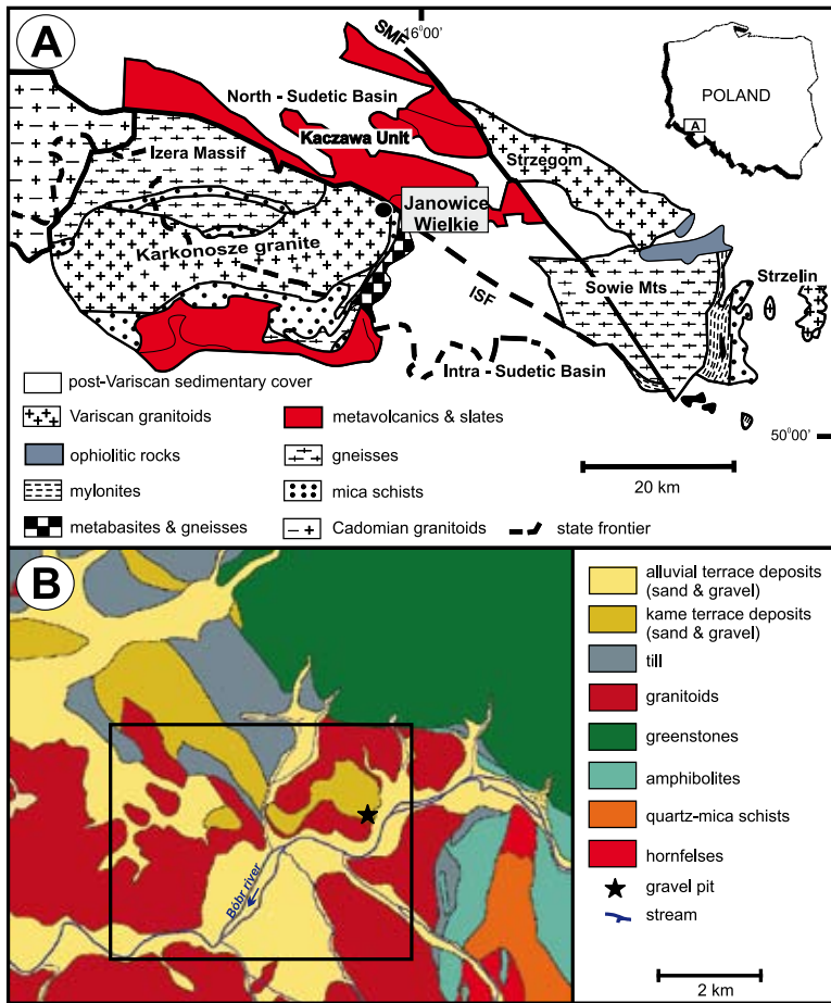
Fig. 1. A - Geological map of the Sudetes Mountains (simplified after Aleksandrowski et al., 1997) with location of the gravel pit in Janowice Wielkie. ISF = Intra-Sudetic Fault, SMF = Sudetic Marginal Fault; B - Geological map of the area around Janowice Wielkie (after Szalamacha, 1956, 1969; partly modified). The rectangle shows the area presented in Fig. 2A.
