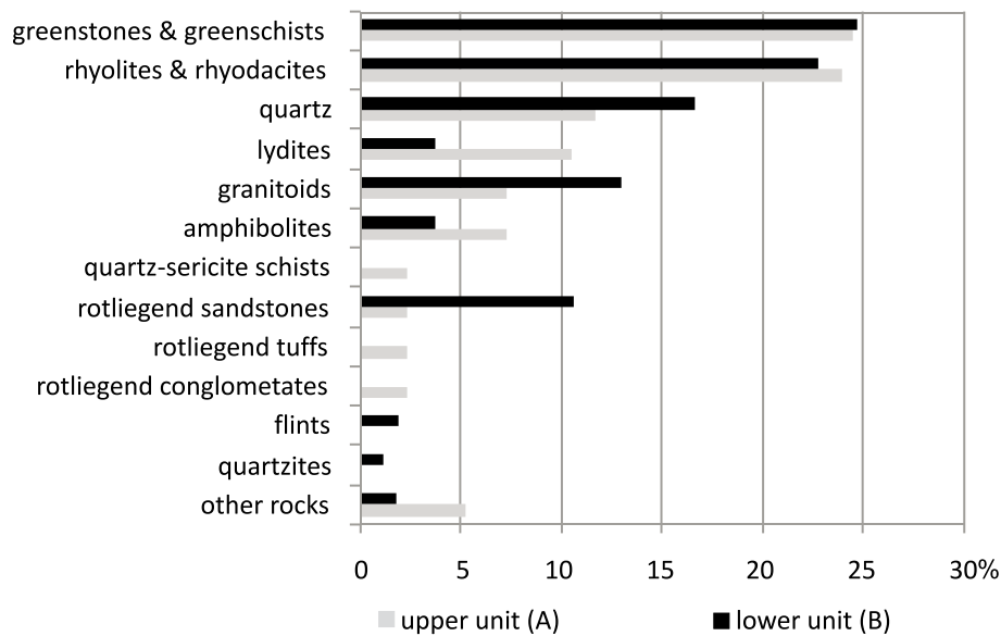
Fig. 5. Petrographical composition of the gravels in the upper (A) and lower (B) units.
