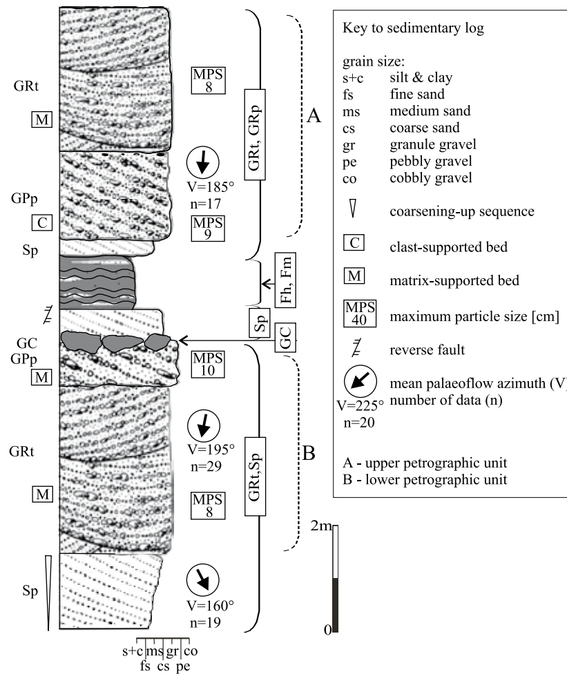
Fig. 4. Sedimentary log from the Janowice Wielkie pit.
