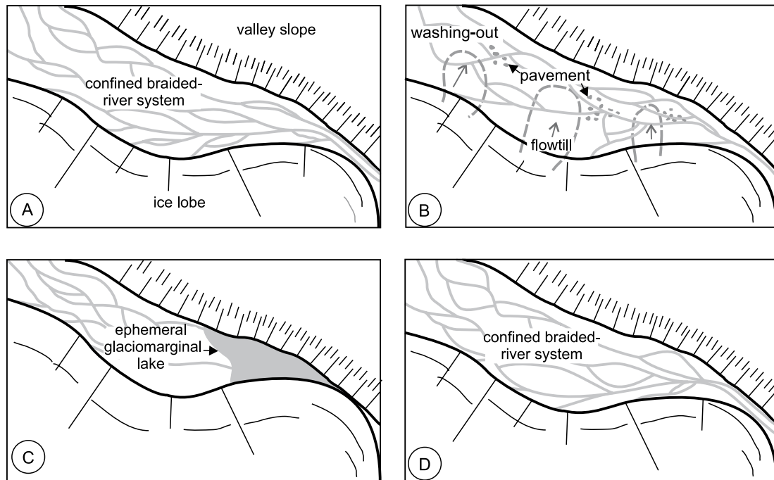
Fig. 6. Schematic model for the kame-terrace sedimentation. A - High-energy, deep channel system of a confined braided river; B - Gravity-induced flowtill and its fluvial reworking; C - Deposition in an ephemeral, small glaciomarginal lake; D - Return to a high-energy, deep channel system of a confined braided river.
