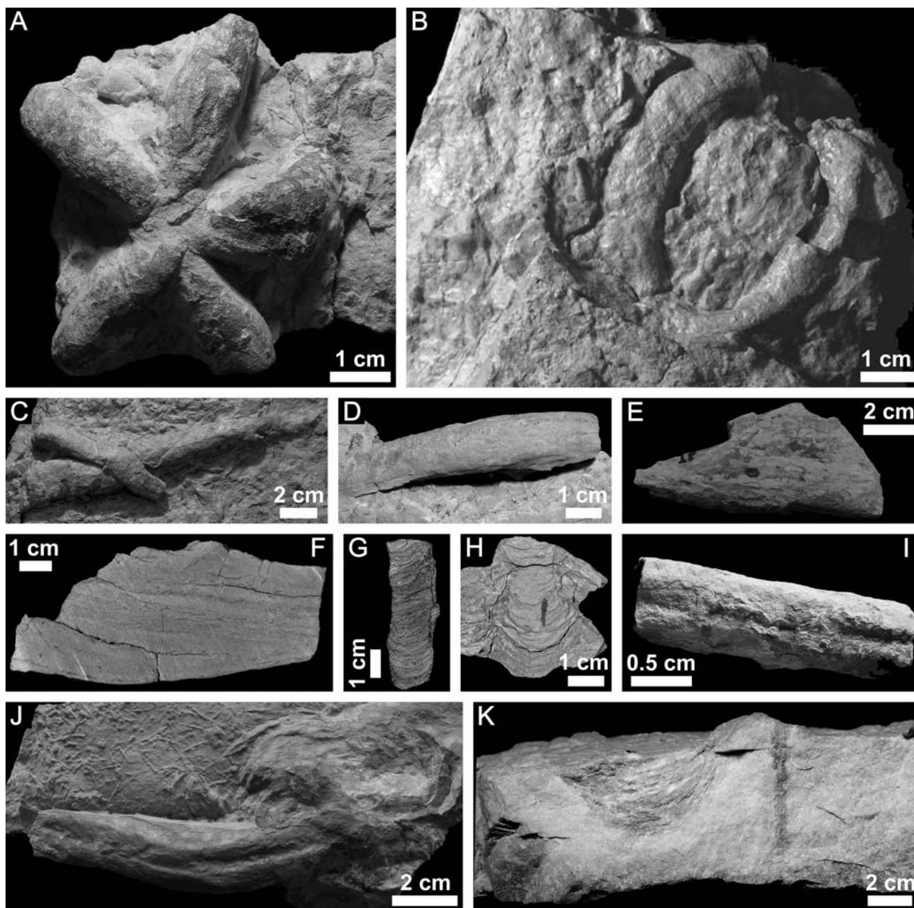
Fig. 15. Radial, spiral and spreite structures from the Ocieseński Formation. A. Dactyloidites asterioides (Fitch, 1850), Hypichnial convex relief in thin wacke bed, INGJ214P/Ig101; Schmidtellus-Holmia Superzone, Igrzyczna. B. Gyrolithes isp., endichnion in thin wacke bed, INGJ214P/Ig96; Schmidtellus-Holmia Superzone, Igrzyczna Hill. C–H. Teichichnus rectus Seilacher, 1955, Schmidtellus-Holmia Superzone; C – hypichnia in thin, bioturbated quartz arenite bed, two overcrossing specimens, INGJ214P/St61, Sterczyna; D – hypichnion in thin quartz arenite bed, INGJ214P/St2, Sterczyna; E – endichnion, side view, INGJ214P/St1, Sterczyna; F – endichnion, cut surface parallel to axis of burrow and bedding plane, INGJ214P/Ig3, Igrzyczna; G – endichnion, cut surface perpendicular to the axis of burrow and bedding plane, INGJ214P/St1a, Sterczyna; H – endichnion, cut surface perpendicular to the axis of burrow and bedding plane, INGJ214P/Ig5, Igrzyczna. I, J. Teichichnus duplex Schlirf and Bromley, 2007, Schmidtellus-Holmia Superzone; I – endichnion in thin wacke bed, INGJ214P/Ig45, Igrzyczna Hill; J – hypichnial full relief in thin quartz arenite bed, on the right side fragment of Cruziana dispar , INGJ214P/Mr90, Igrzyczna Hill. K. Diplocraterion parallelum Torell, 1870, endichnion in thin quartz arenite bed, INGJ214P/Ig130, Schmidtellus-Holmia Superzone, Igrzyczna Hill.
