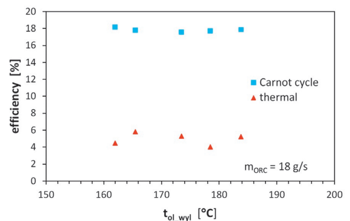
Fig. 5. Performance characteristics of ethyl alcohol vapour cycle
