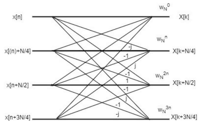
Fig. 1. Basic Radix-4 structure
