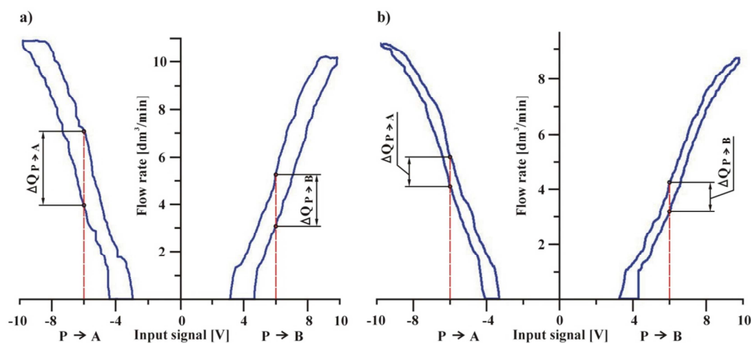
Fig. 2. Static characteristics of the proportional directional control valve (type DIFB): a) without Dither control, b) with the Dither control
