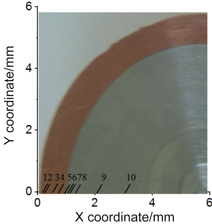
Fig. 7. Radius coordinate diagram of measuring points
