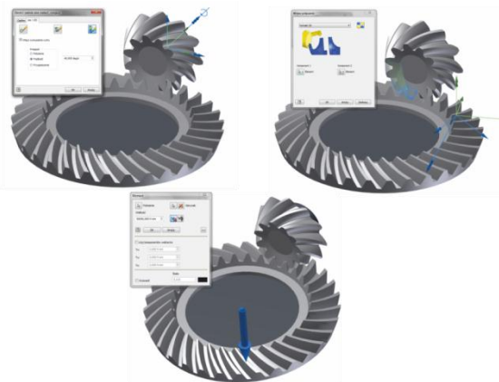
Fig. 5. Bevel gearbox solid model in the dynamic simulation environment
