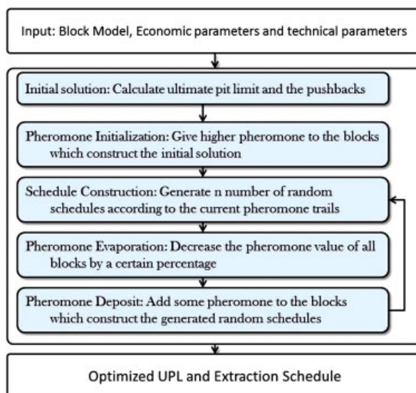
Fig. 2. The process of long-term open-pit production planning using ACO
