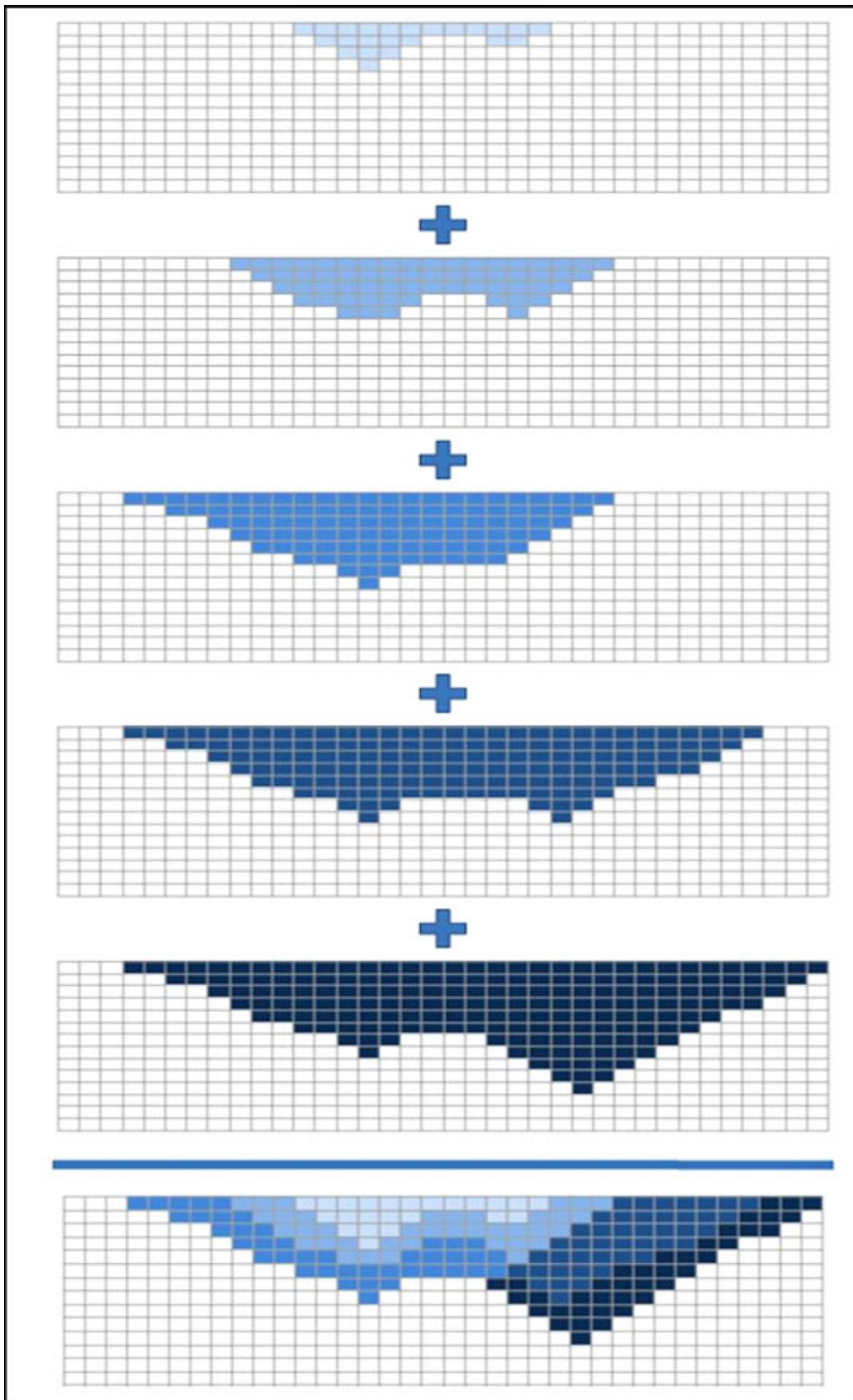
Fig. 6. Combination of generated pits to produce a mine schedule
