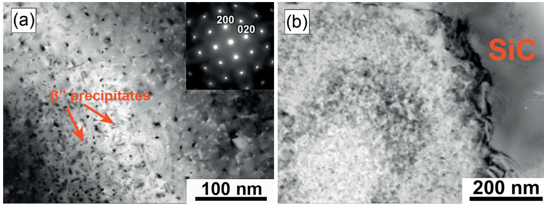
Fig. 5. TEM micrographs of AA6061-5 vol. % SiC p composite, a) needle-shape β'' precipitates, b) microstructure close to matrix-particle interface
