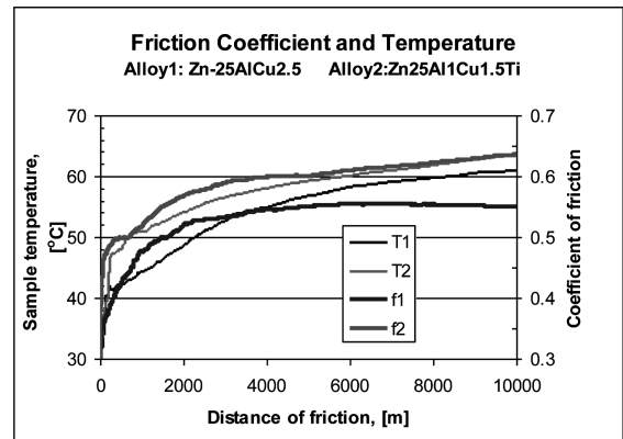
Fig. 5. Coefficient of friction and sample temperature during sliding wear tests. The samples were aged naturally for 5 years after casting
