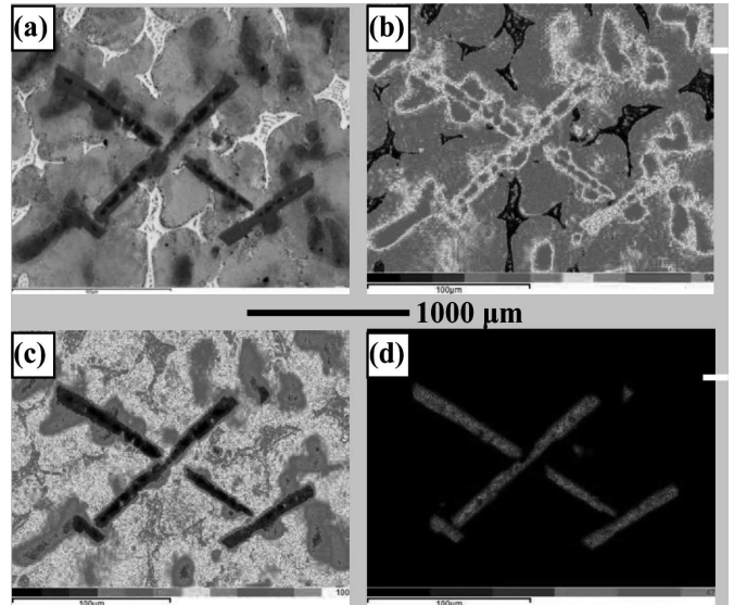
Fig. 3. SEM back-scattered electron images of the Zn-26Al-1.6Ti alloy (a) and surface distribution of Al (b), Zn (c) and Ti (d) [10]
