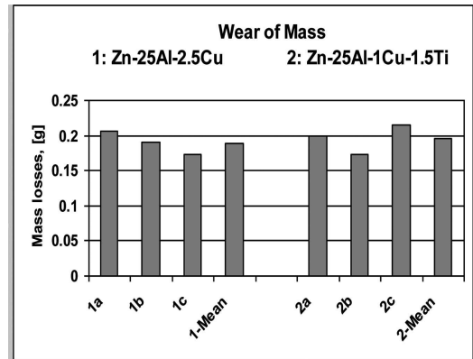
Fig. 4. Mass losses of the samples after 10 km distance of sliding wear test. The samples were aged naturally for 5 years after casting
