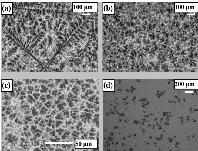
Fig. 1. Examples of Zn-25 Al alloy microstructures. (a) LM picture of initial coarse dendritic alloy (b) LM picture of alloy inoculated with Zn-4Ti grain refiner (0.05 wt.% Ti); (c) alloy Zn-25Al; (c) and (d) SEM and LM pictures of alloy Zn-25Al-1Cu-2Ti (visible Ti(Al,Zn) 3 reinforcing particles) [1, 2]
