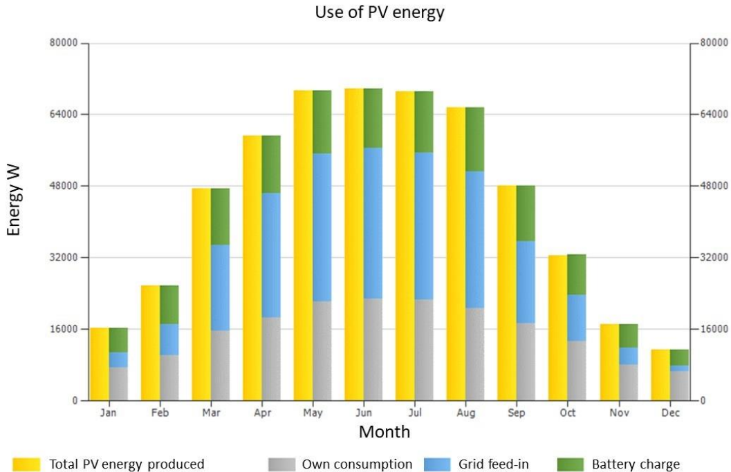
Figure 9. Graph of the use of PV energy in the warehouse (PV*Sol). Source: Own.
