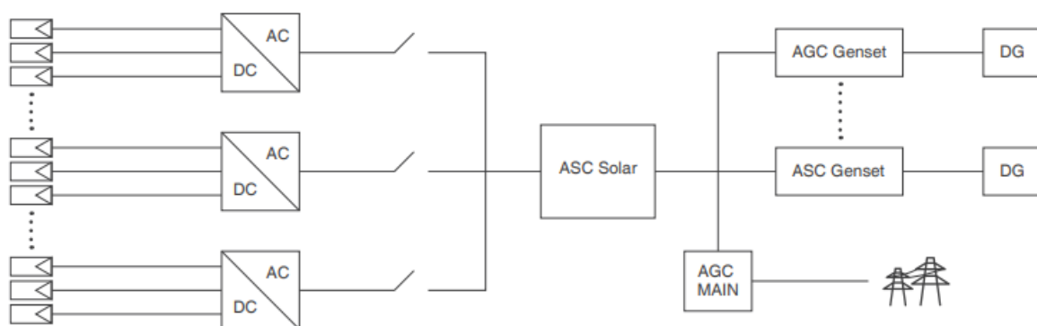
Figure 3. Backup generator scheme. Source: [14].
