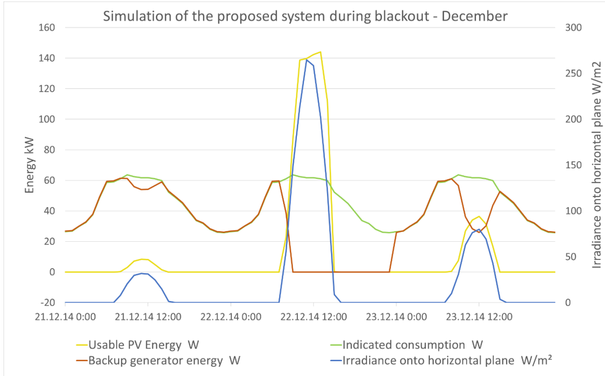
Figure 10. Use of backup generator during low-irradiation days (PV*Sol). Source: Own.
