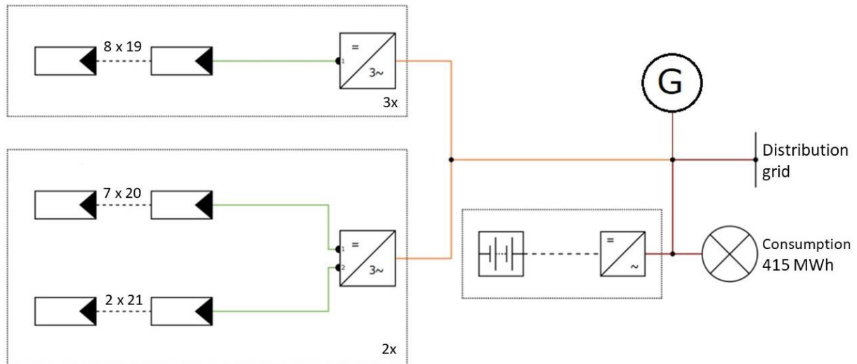
Figure 4. Schematic diagram of the proposed system. Source: Own.
