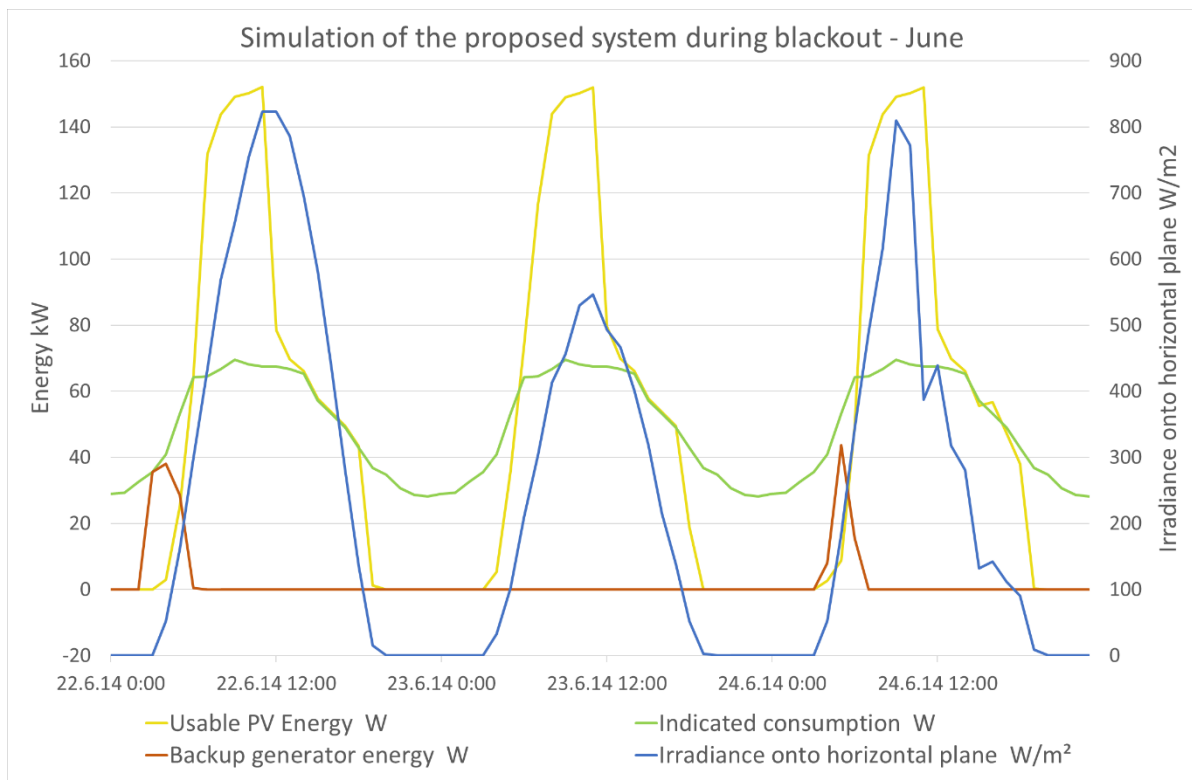
Figure 11. Use of backup generator during high-irradiation days (PV*Sol). Source: Own.
