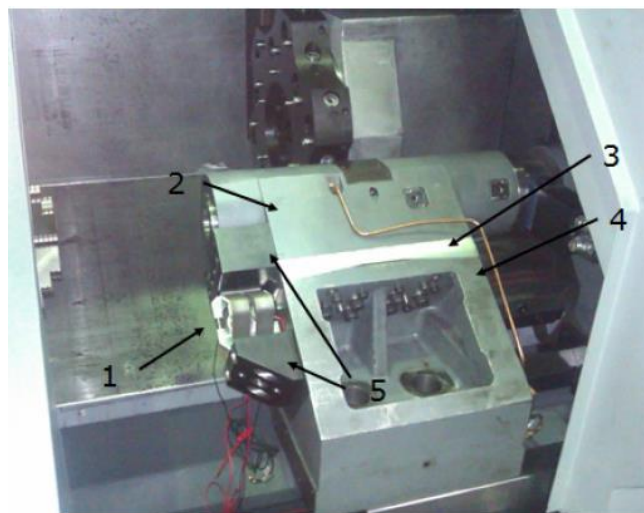
Fig. 9. The Joint Interface Module incorporated in the tailstock of the lathe
