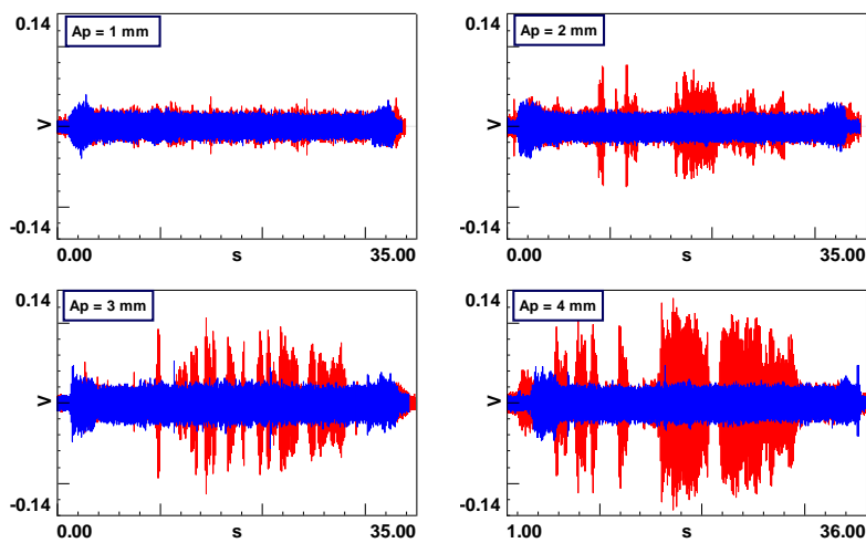
Fig. 13. Time domain microphone signal from the cutting processes. Red: Reference tool holder, Blue: JIM tool holder. Using the JIM tool holder allowed for machining in stable conditions with increased depth of cut as compared to the reference tool holder
