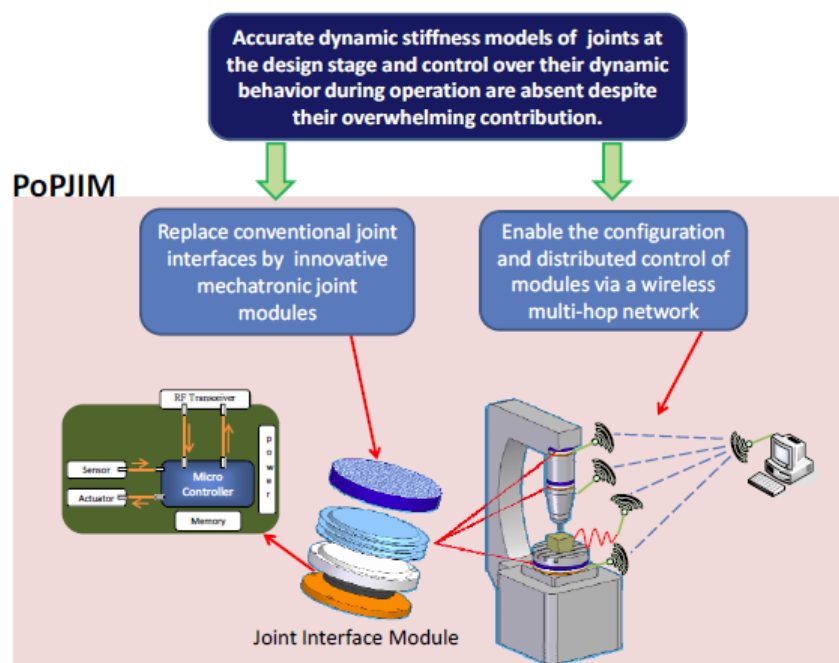
Fig. 7. Joint interface module for controlling the static and dynamic behaviour
