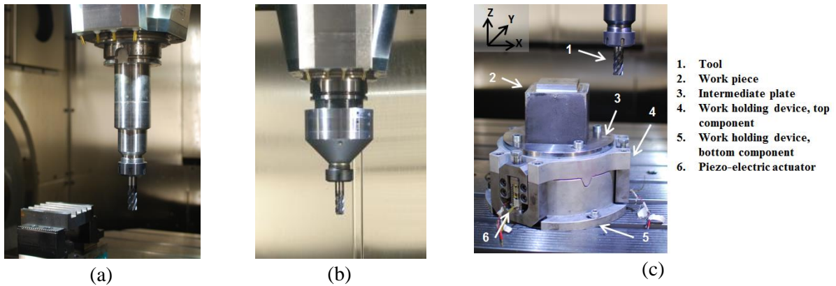
Fig. 12. JIM prototypes for controlling the milling machine; (a) Passive JIM tool holder, (b) Active JIM tool holder, (c) Active JIM workholding device
