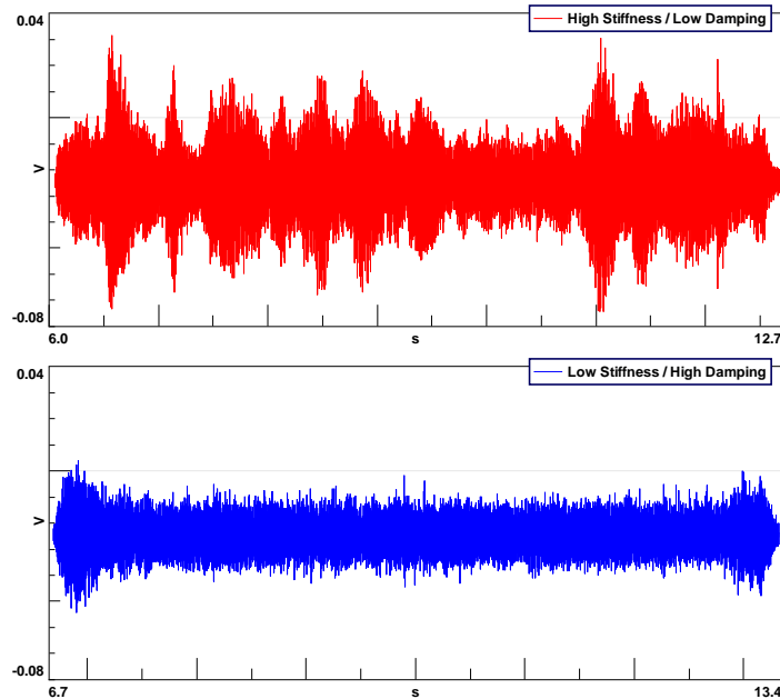
Fig. 15. Time domain microphone signal from the machining process with the JIM preset at the two air pressure configurations. Top: high stiffness/low damping, Bottom: low stiffness/high damping
