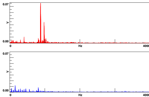
Fig. 14. Frequency domain microphone signal from the cutting processes. Red: Reference tool holder, Blue: JIM tool holder. The Chatter frequency resides at approximately 880 Hz
