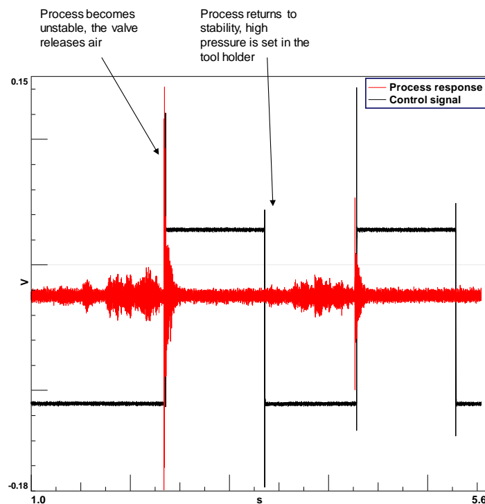
Fig. 17. Time domain signal of the process response and the control system voltage supplied to activate the valve
