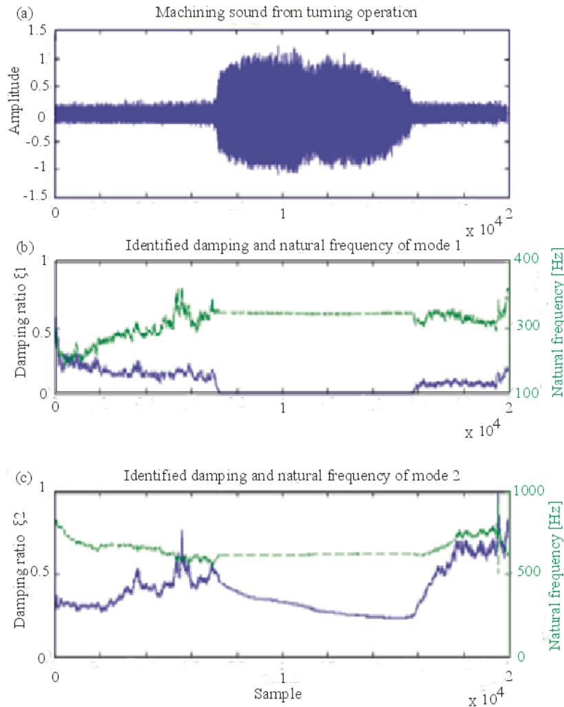
Fig. 6. In-process identification and modelling of damping and natural frequency in turning [19]. Sound pressure level measured by a microphone (a), Identified first natural frequency and damping ratio (b), Identified second natural frequency and damping ratio (c)
