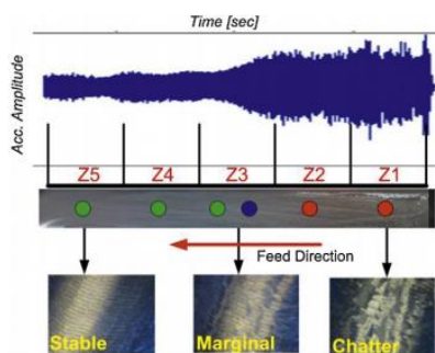
Fig. 1. Accelerometer data and surfaces of stable and chatter zones [5]
