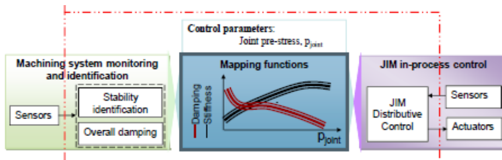
Fig. 8. Control architecture of the Joint Interface Modules (JIM)
