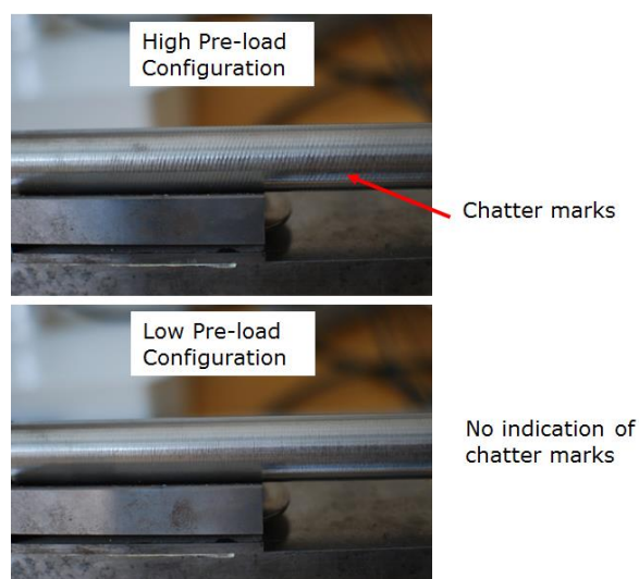
Fig. 11. Comparison of the surface of the bars machined in the high pre-load configuration (upper) and low pre-load configuration (lower)
