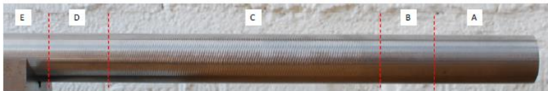
Fig. 10. Machined bar final diameter of 24 mm, high pre-load configuration. As the process was unstable, distinctive chatter marks appear on the surface
