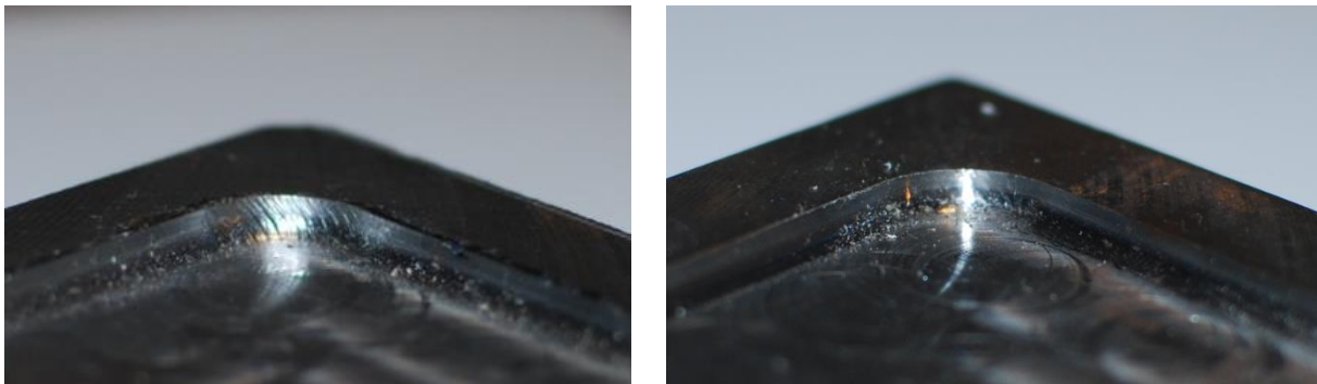
Fig. 16. The corner of the machined pocket with the tool holder at high stiffness/low damping configuration (left) and low stiffness/high damping configuration (right)
