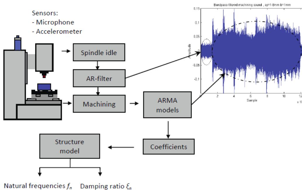
Fig. 4. ARMA model identification [19]
