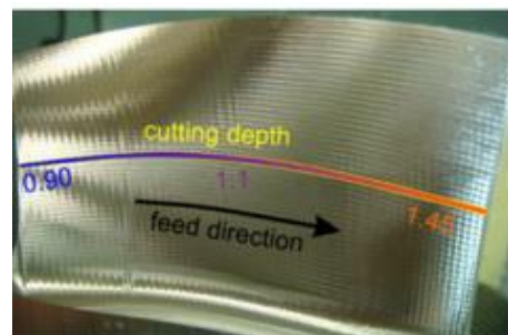
Fig. 2. Chatter marks in milling [4]
