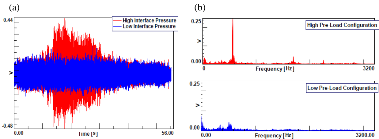
Fig. 12. Comparison of microphone signals acquired during machining with high preload (red) and low pre-load (blue) – time domain: The amplitude of the signal increases sharply as the process becomes unstable (a), The distinctive chatter frequency lies around 560 Hz (b)
