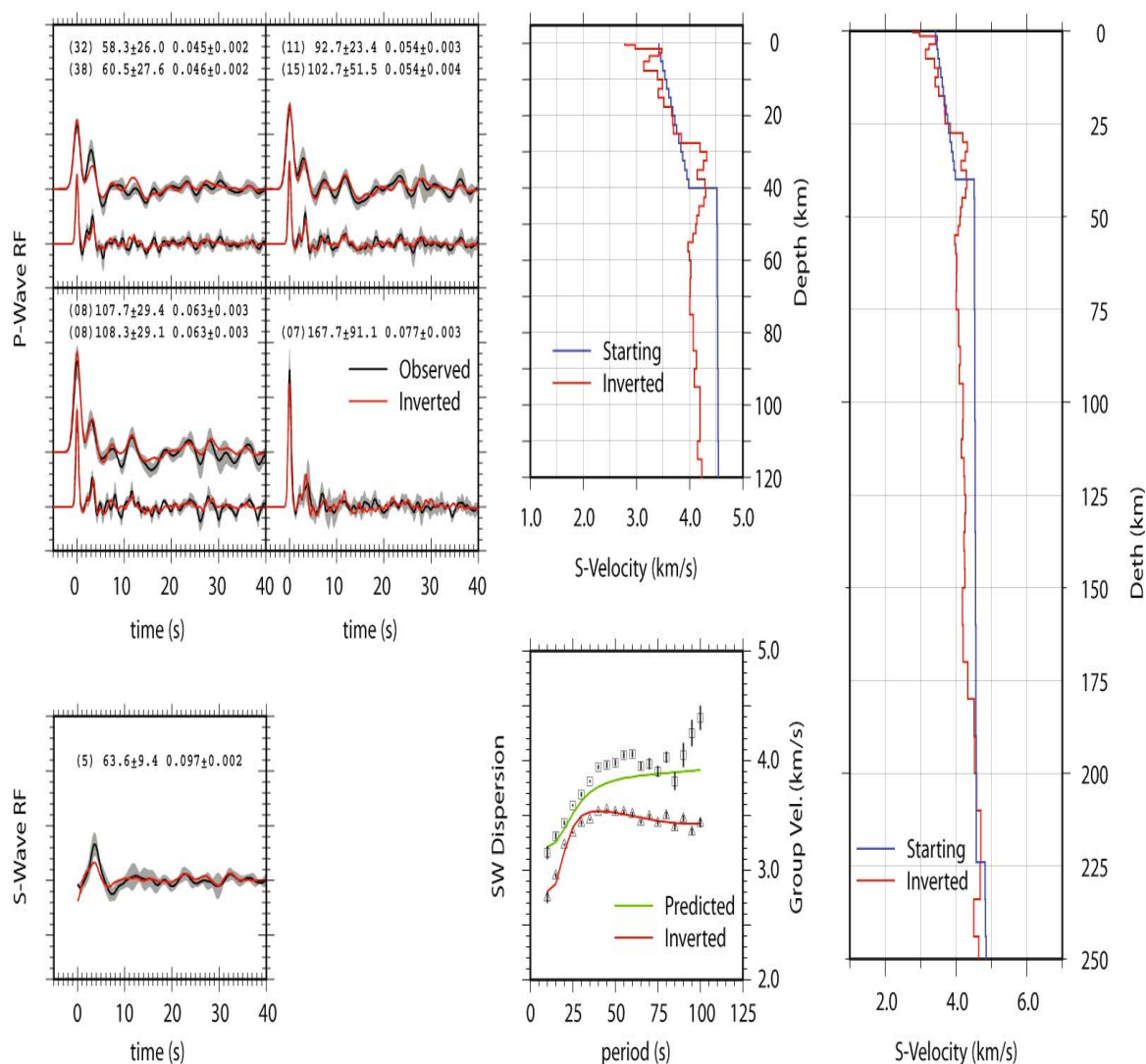
Text-fig. 6. Joint inversion of PRFs, SRFs, and SW dispersion velocities at station AYUS. The left panels display observed (black) and predicted (red) receiver functions and the middle panel at the bottom displays observed (symbols) and predicted (lines) group velocities. Only fundamental-mode, Rayleigh waves were used during the inversion (red) but a prediction for the fundamental-mode, Love-wave, group velocity is shown (green). The inverted S-velocity model is shown to the right, with the crustal portion enlarged in the middle (top) panel
