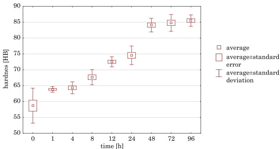
Fig. 2. Changes in element hardness as a function of irradiation time
