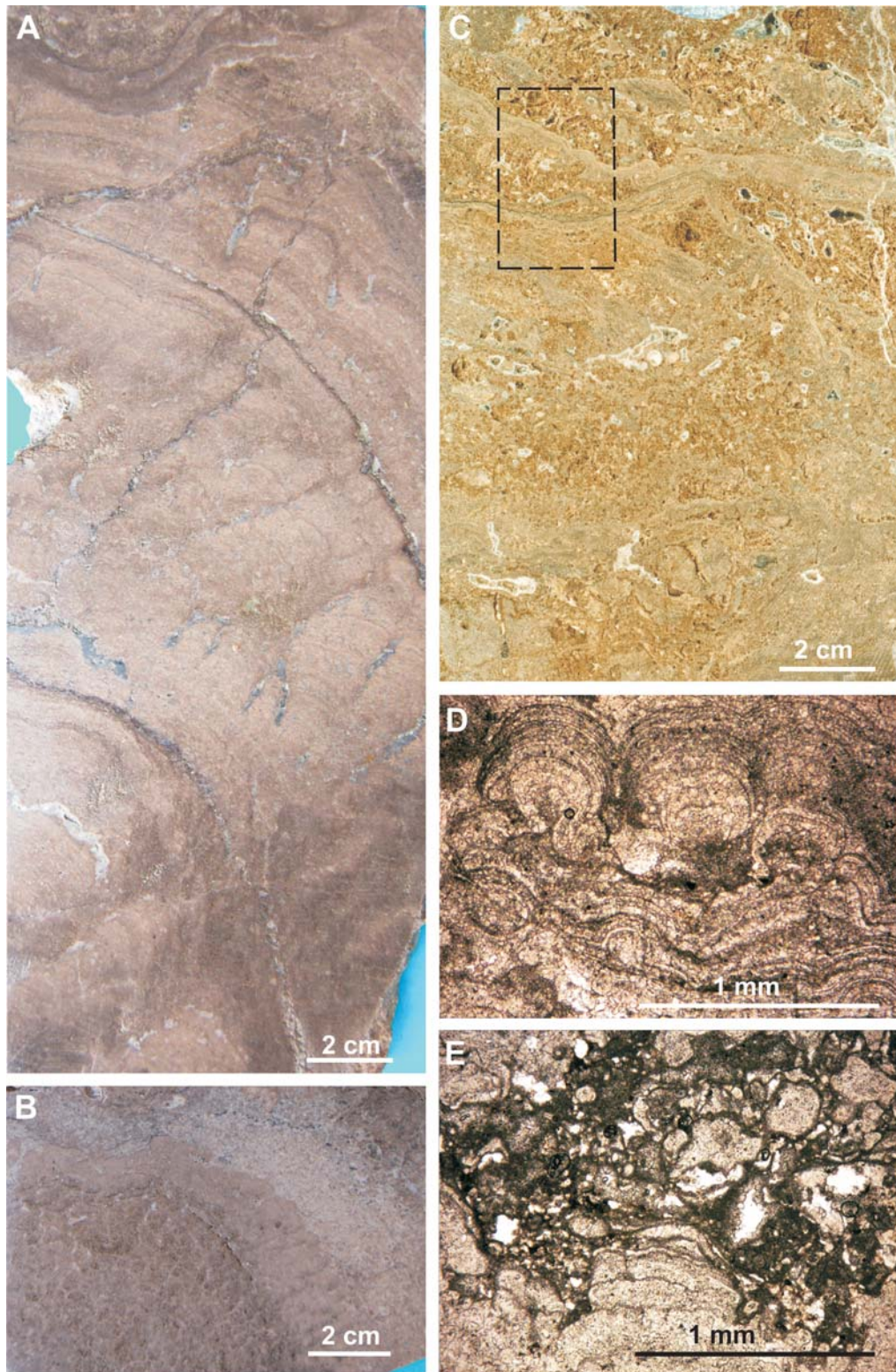
Fig. 10. Stromatolites. A, B. Columnar stromatolites of variable inclination of columns, eventually passing into planar forms (A – Jabłonna 1; B – Jabłonna 3). C, E. Recrystallized, granular deposit with common subhorizontal microbial planar encrustations (Jabłonna 3). The dotted quadrangle in C shows the place of thin section, parts of which are shown in D (thinly-laminated microdomes and mats) and E (more vaguely laminated stromatolite).
