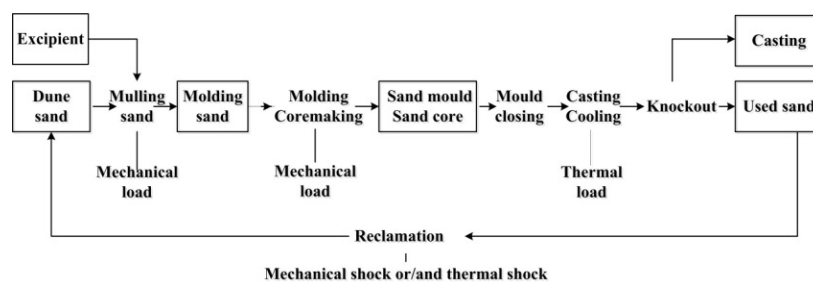
Fig. 1. The foundry sand service process
