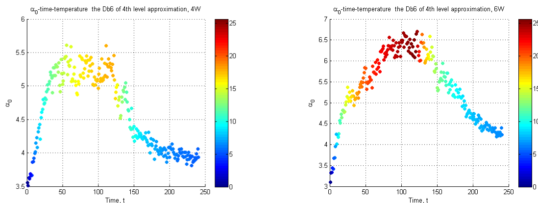
Fig. 9. Dependence of the shape parameter on time and temperature, for experiments with two powers of heating transducer, left image corresponds to the power of 4 W applied to the transducer and the right image corresponds to the power of 6 W.
