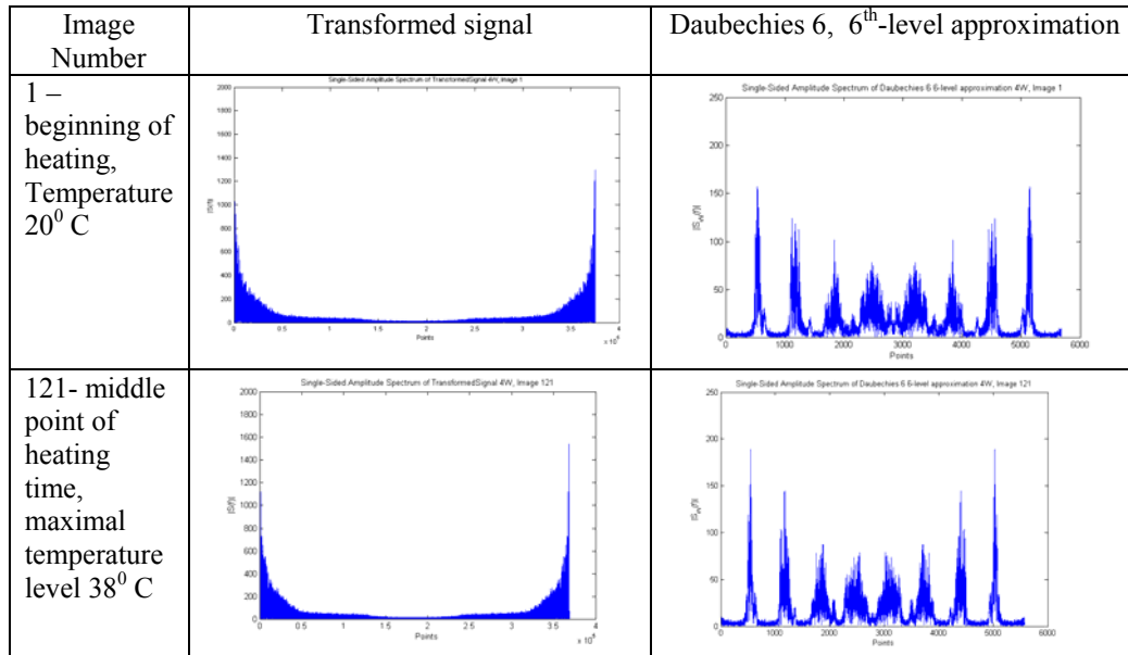
Fig 10. FFT transforms of signal and wavelet approximations.
