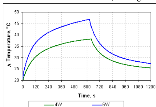
Fig. 2. The experimentally determined by thermocouples temperature changes at the point of focus (the highest heating) in the pork loin sample as a function of time / different values of power applied to the 4 and 6 W transducer, 10 min heating and 10 min cooling.
