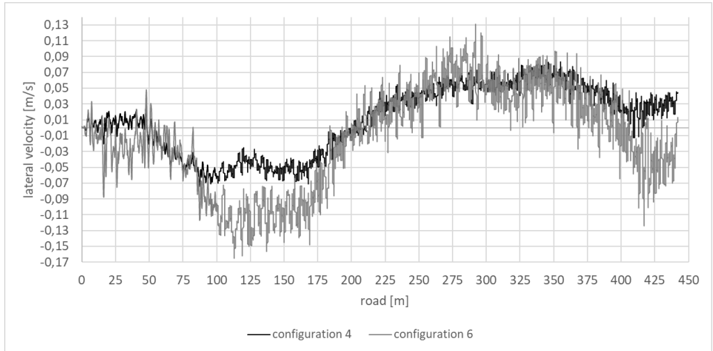
Fig. 8. Lateral velocity on an icy, randomly uneven road surface with the almost similar left and right profiles of irregularities ( cor_H = 0.8 ) [own research]
