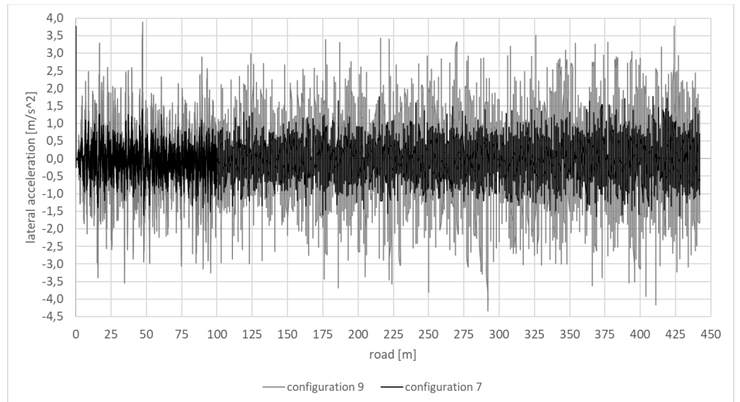
Fig. 13. Lateral acceleration on a dry, randomly uneven road surface with the almost different left and right profiles of irregularities ( cor_{rl} = 0.2 ) [own research]
