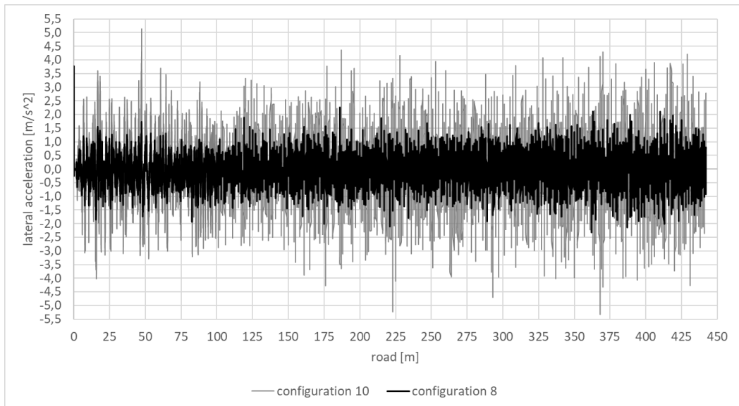
Fig. 14. Lateral acceleration on an icy, randomly uneven road surface with the almost different left and right profiles of irregularities ( cor_{rl} = 0.2 ) [own research]
