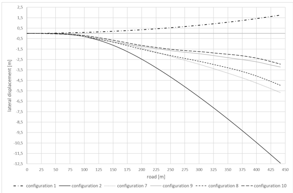
Fig. 4. Trajectories on a dry and icy as well as flat and randomly uneven road surface with the almost different left and right profiles of the irregularities ( cor_H = 0.2 ) [own research]
