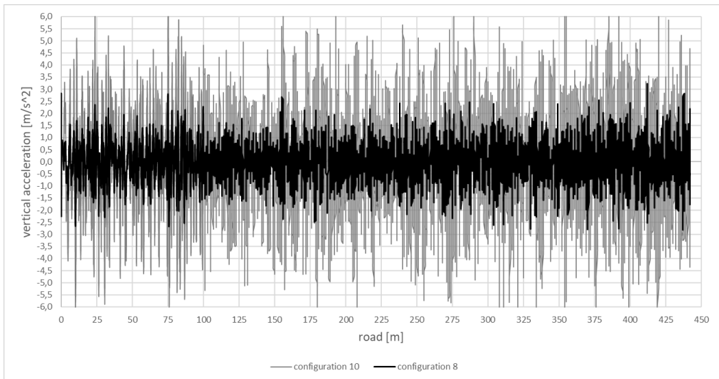
Fig. 19. Vertical acceleration on an icy, randomly uneven road surface with the almost different left and right profiles of irregularities as well as different amplitudes of these irregularities [own research].
