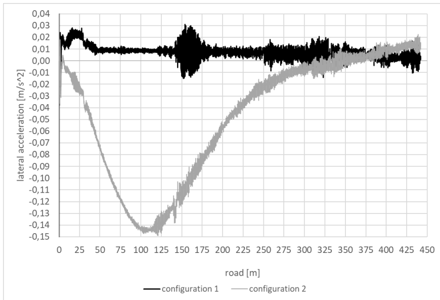
Fig. 10. Lateral acceleration on a dry and an icy flat road surface [own research]
