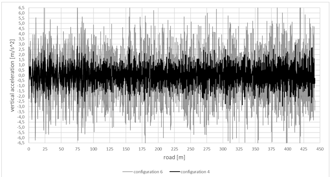
Fig. 17. Vertical acceleration on an icy, randomly uneven road surface with the almost similar left and right profiles of irregularities as well as different amplitudes of these irregularities [own research].
