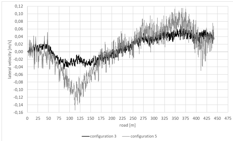
Fig. 7. Lateral velocity on a dry, randomly uneven road surface with the almost similar left and right profiles of irregularities ( cor_H = 0.8 ) [own research]
