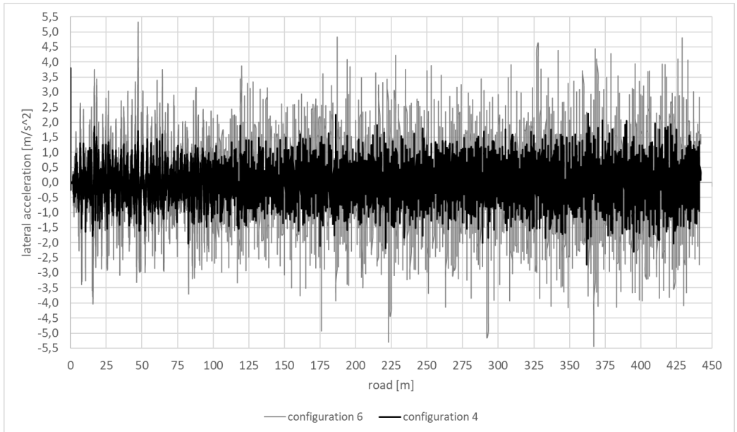
Fig. 12. Lateral acceleration on an icy, randomly uneven road surface with the almost similar left and right profiles of irregularities ( cor_{rl} = 0.8 ) [own research]
