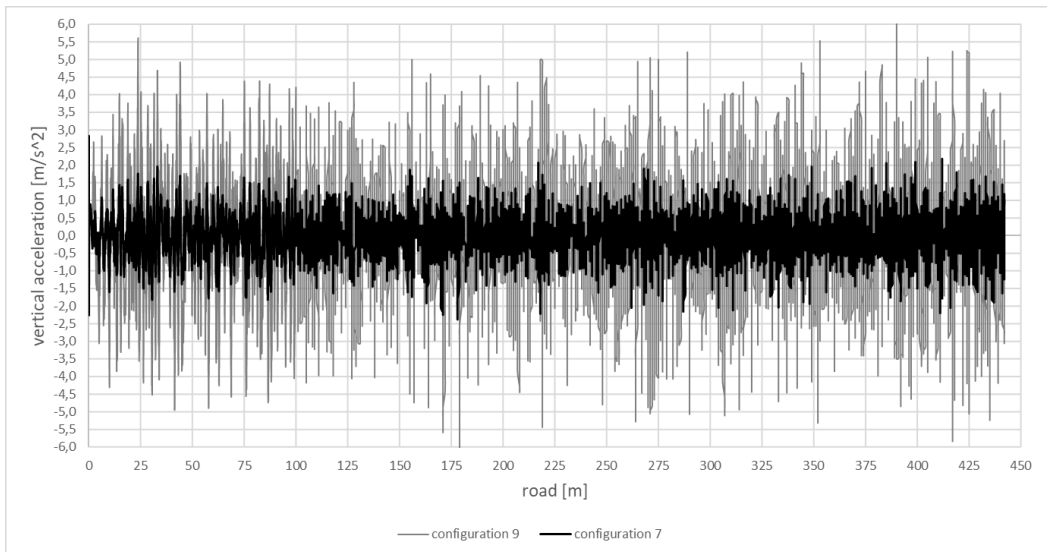
Fig. 18. Vertical acceleration on a dry, randomly uneven road surface with the almost different left and right profiles of irregularities as well as different amplitudes of these irregularities [own research].
