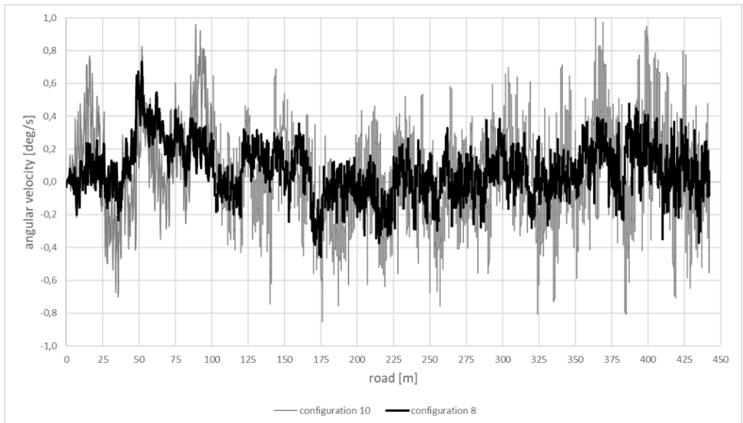
Fig. 24. Angular velocity around the vertical axis on an icy, randomly uneven road surface with the almost different left and right profiles of irregularities as well as different amplitudes of these irregularities [own research].
