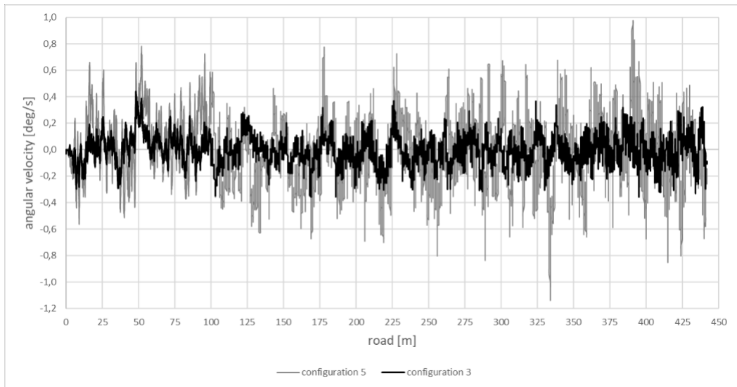
Fig. 21. Angular velocity around the vertical axis on a dry, randomly uneven road surface with the almost similar left and right profiles of irregularities as well as different amplitudes of these irregularities [own research].
