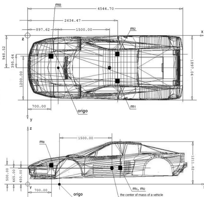
Fig. 2. Location of the additional masses in the vehicle's body and the 'origo' point (Kisilowski, 2019)
