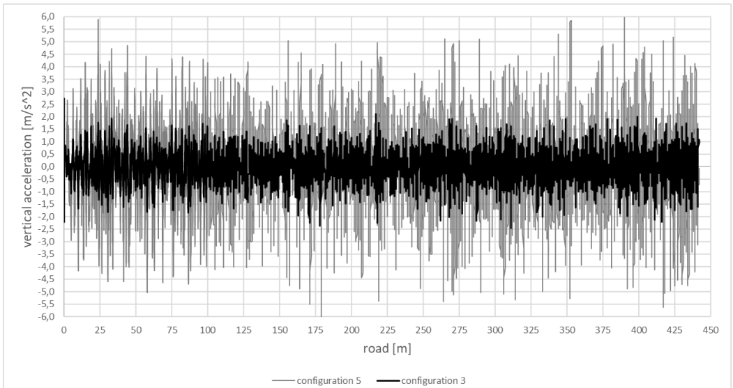
Fig. 16. Vertical acceleration on a dry, randomly uneven road surface with the almost similar left and right profiles of irregularities as well as different amplitudes of these irregularities [own research].
