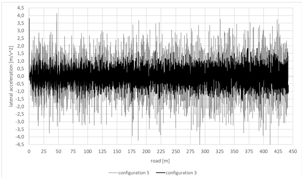
Fig. 11. Lateral acceleration on a dry, randomly uneven road surface with the almost similar left and right profiles of irregularities ( cor_H = 0.8 ) [own research]
