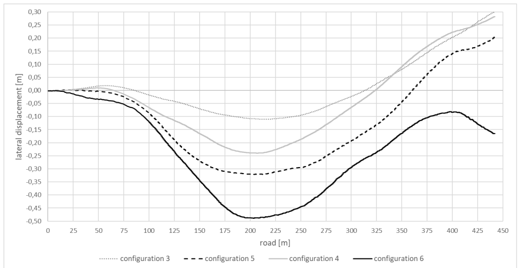
Fig. 5. Trajectories on an icy and randomly uneven road surface with the almost similar left and right profiles of the irregularities ( cor_H = 0.8 ) [own research]
