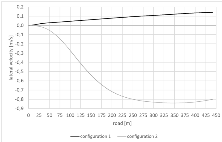
Fig. 6. Lateral velocity on a dry and icy flat road surface [own research]
