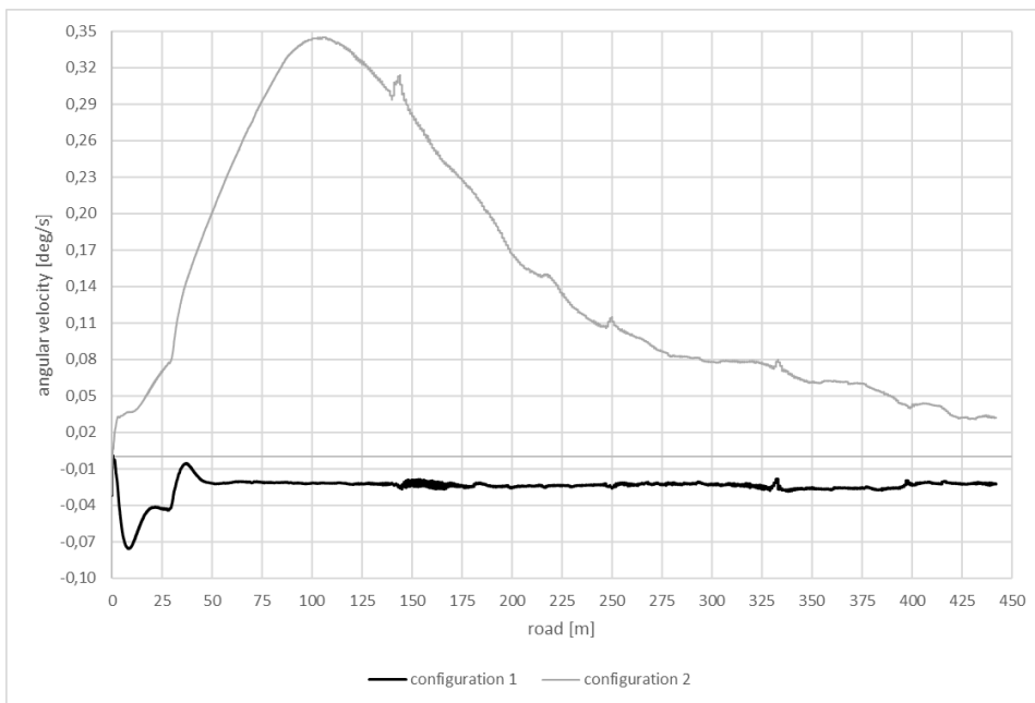
Fig. 20. Angular velocity around the vertical axis for the motion on a dry and icy flat road [own research].
