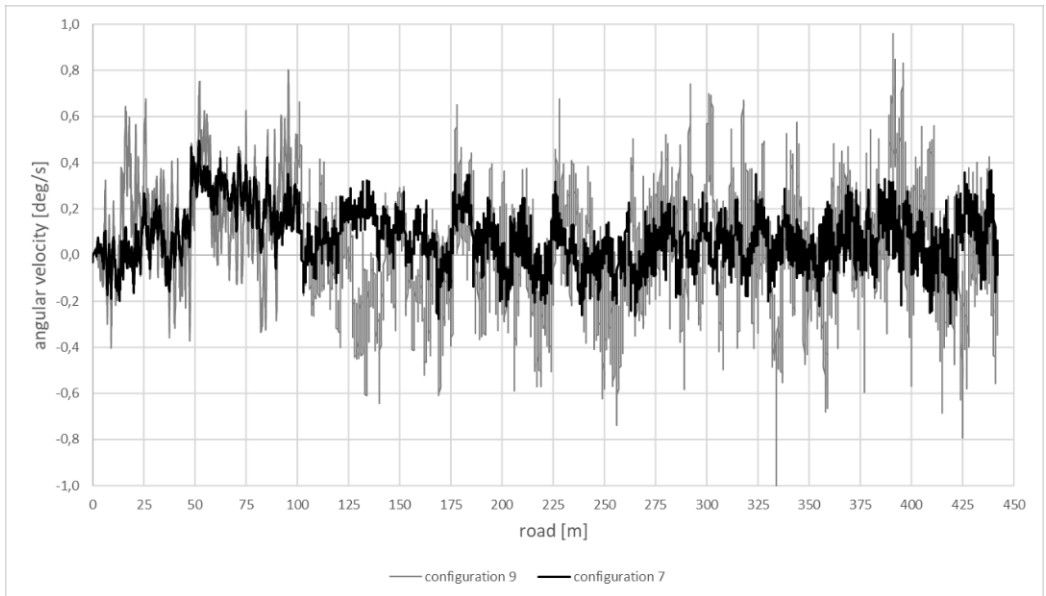
Fig. 23. Angular velocity around the vertical axis on a dry, randomly uneven road surface with the almost different left and right profiles of irregularities as well as different amplitudes of these irregularities [own research].
