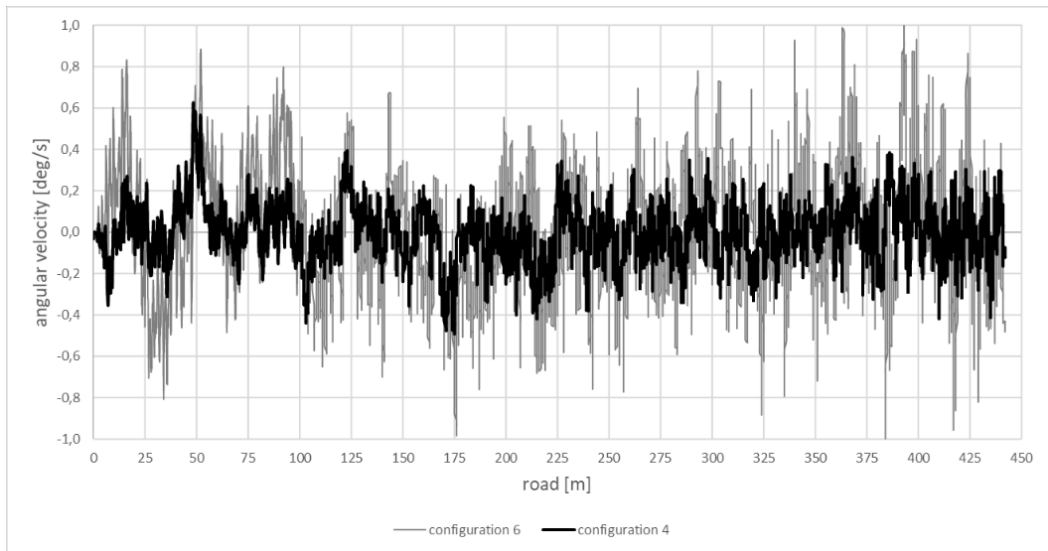
Fig. 22. Angular velocity around the vertical axis on an icy, randomly uneven road surface with the almost similar left and right profiles of irregularities as well as different amplitudes of these irregularities [own research].
