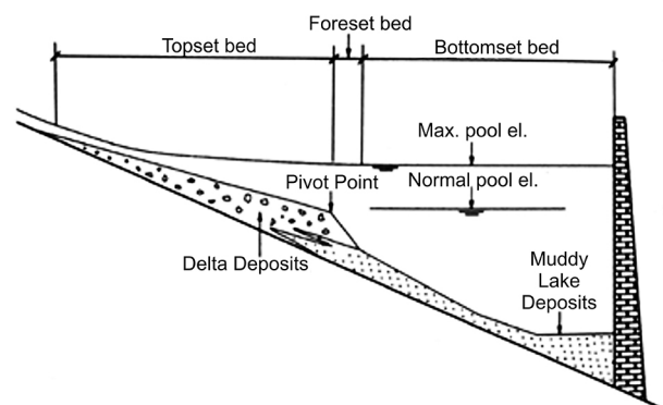
Fig. 1. Longitudinal profile showing typical variation in sediment characteristics along the length of a reservoir (Morris & Fan, 1998; used with the authors' permission).
