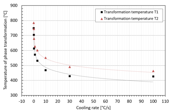
Fig. 7 Dependence of the phase change temperature on the cooling rate
