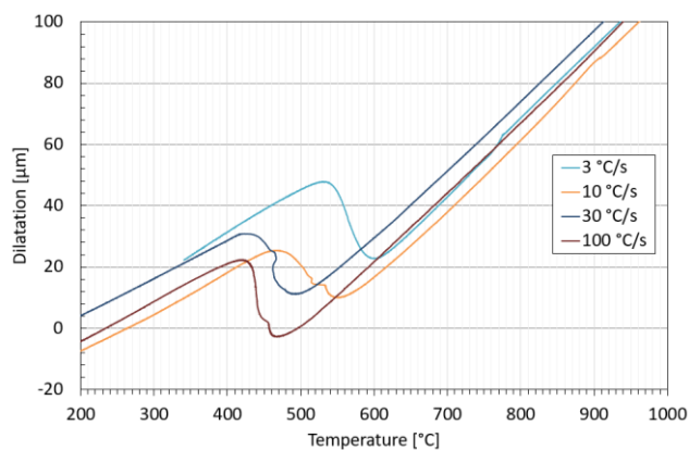
Fig. 4 Detail of the dilatometric curve cooling part for rate 3°C/s; 10°C/s; 30°C/s and 100°C/s
