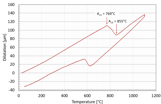
Fig. 2 Complete cycle of dilatometric curve for 1°C/s cooling rate
