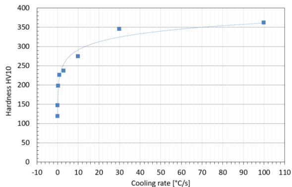
Fig. 8 Dependence of the hardness on the cooling rate
