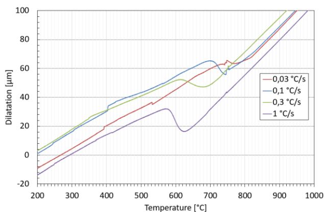
Fig. 3 Detail of the dilatometric curve cooling part for rate 0,03°C/s; 0,1°C/s; 0,3°C/s and 1°C/s
