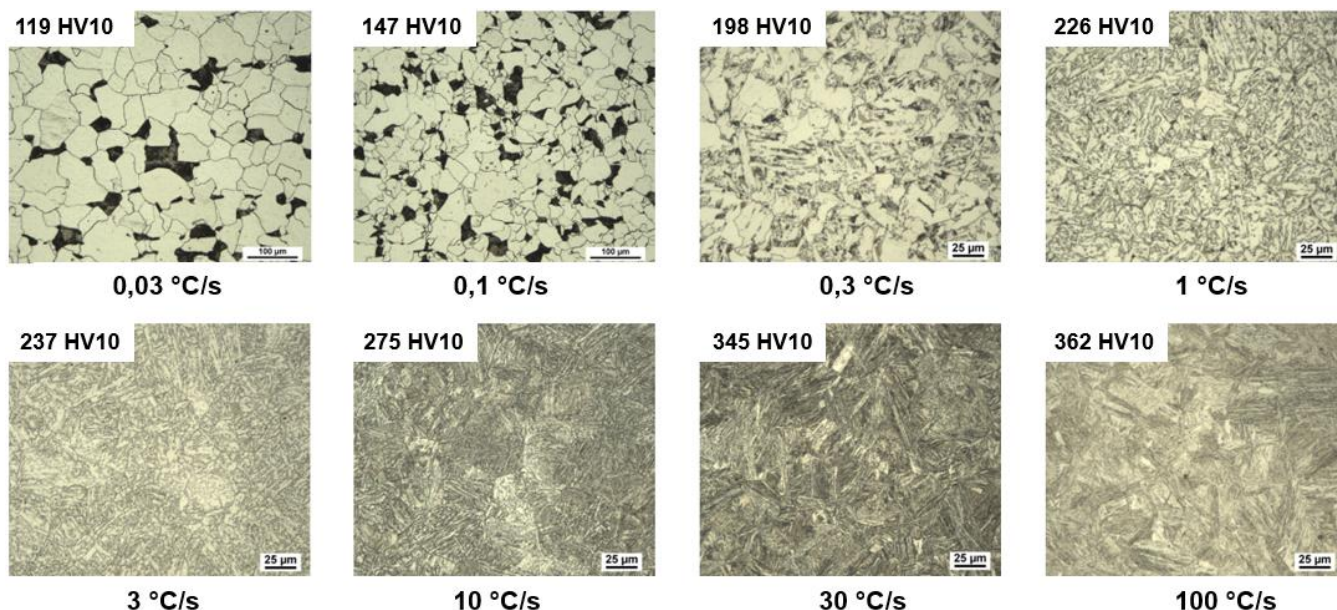
Fig. 9 Microstructures with corresponding cooling rate and hardness
