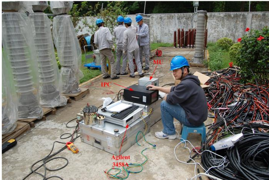
Fig. 11. The picture of on-site calibration in Sanxiang substation.
