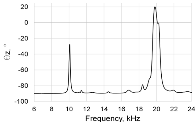
Fig. 3. Impedance of designed burst type signal generator
