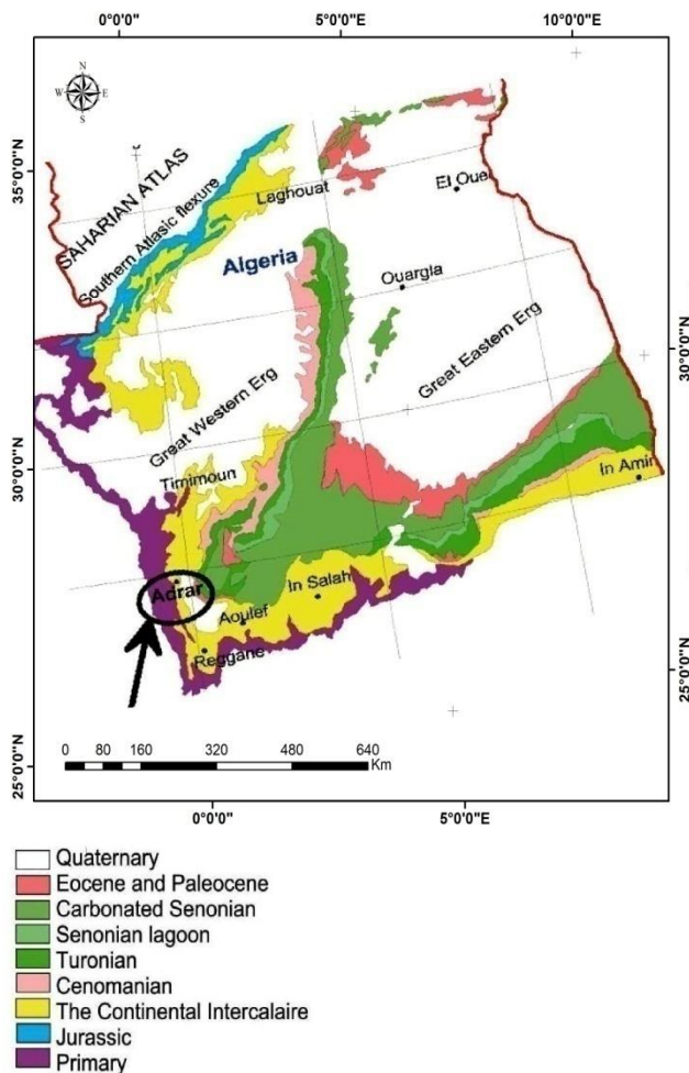
Fig. 4. Geological map of the northern Sahara aquifer system in Algeria; source: KHELFAOUI et al. [2020], modified
