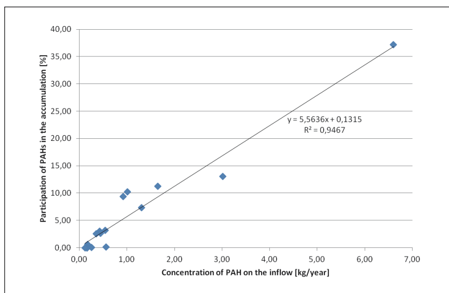
Fig. 3. The correlation between PAH concentration on the inflow and their percentage share in the accumulation
