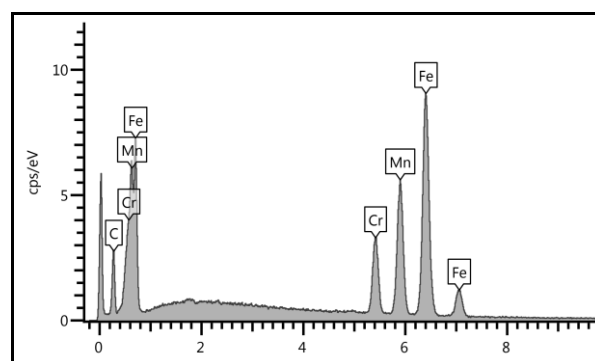
Fig. 5. Sample X-ray spectrum of point 3 in Figure 4
