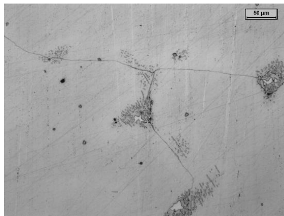
Fig. 3. Microstructure of the GX120MnCr18-2 cast steel, light microscope, nital etching
