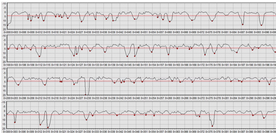
Fig. 3. Unevenness of road pavement in a form of a profile
