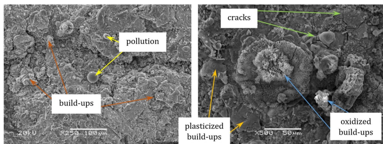
Fig. 6. Sample SEM images of the wear products on the front suspension beam surface
