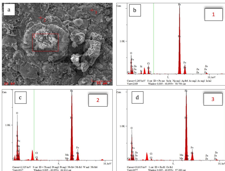
Fig. 8. Spot analysis of the chemical composition: a) SEM image, b) radiation spectrum peculiar for point 1, c) radiation spectrum peculiar for point 2, d) radiation spectrum peculiar for point 3
