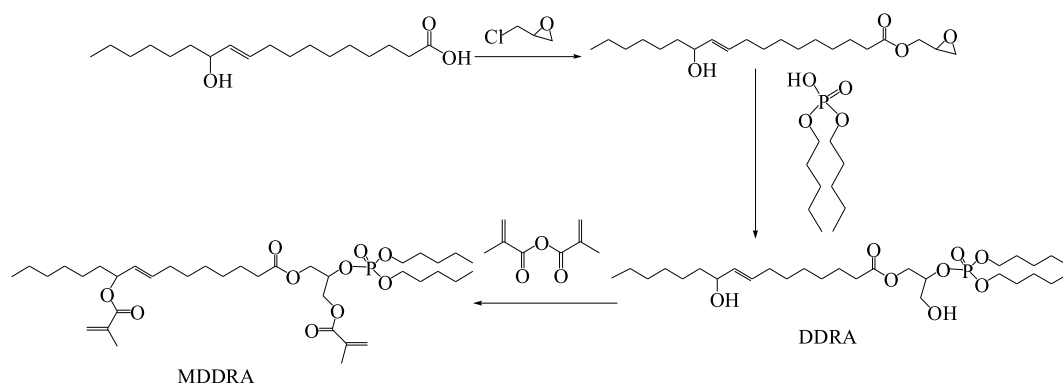
Figure 4. The synthesis route of MDDRA resin monomer
