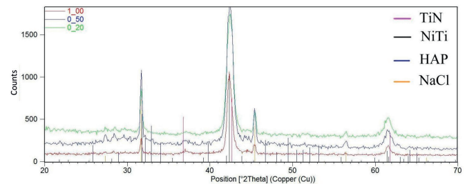
Fig. 8. GIXD patterns measured at incidence angle of 0.3^\circ for the nitrided NiTi alloy with deposited hydroxyapatite layer
