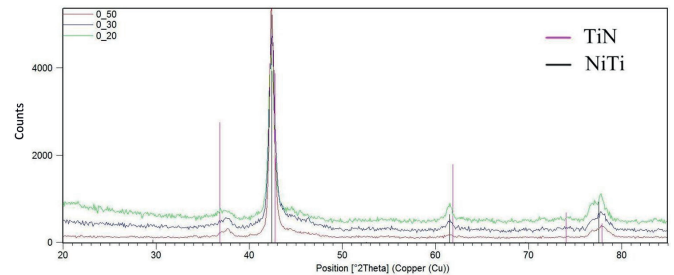
Fig. 1. The GIXD patterns measured at incidence angle of 0.2, 0.3 and 0.50 for layer deposited at 300°C for 30 min
