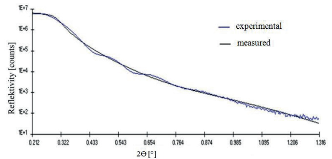
Fig. 2. The reflectivity curve (measured and experimental) for the nitrided layer deposited at 300°C for 30 min
