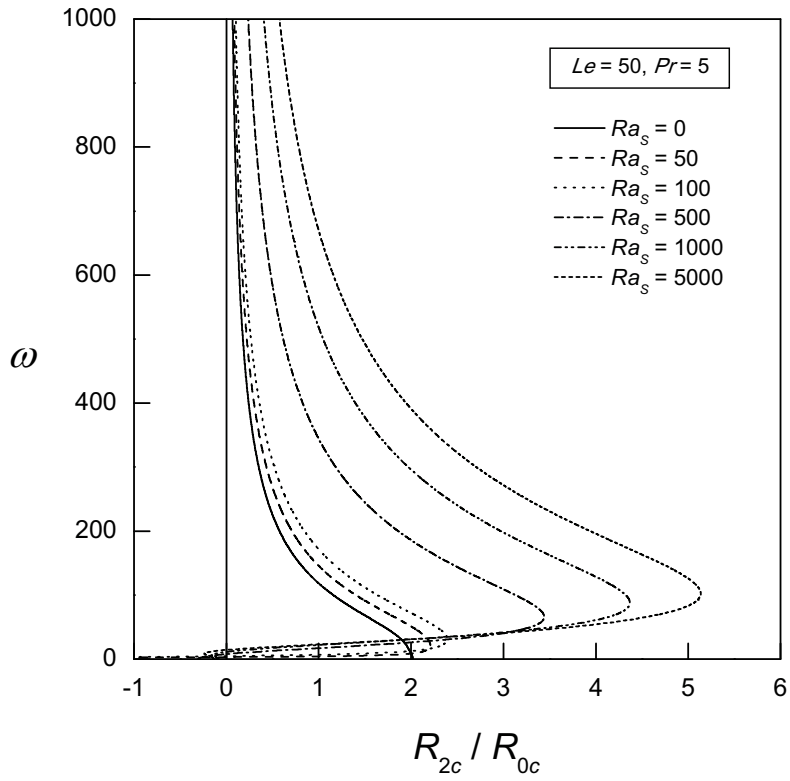
Fig.1. Variation of R_{2c} with \omega for different values of Ra_s .
