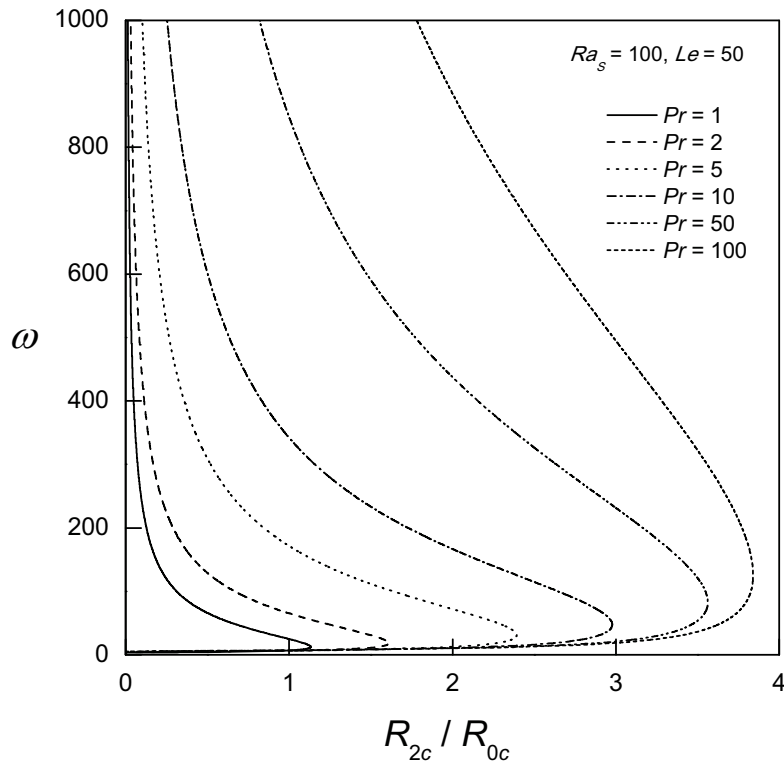
Fig.3. Variation of R_{2c} with \omega for different values of Pr.
