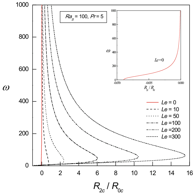
Fig.2. Variation of R_{2c} with \omega for different values of Le .
