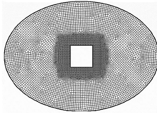
Fig.2. Grid distribution.
