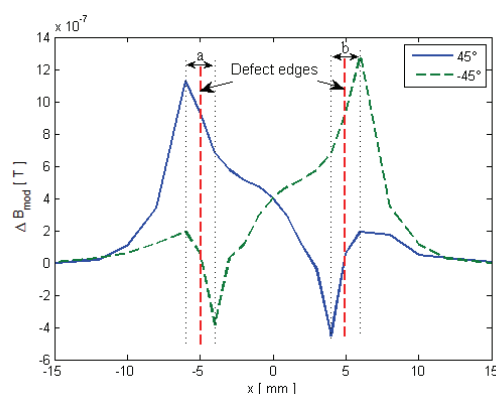
Fig. 6. Numerical simulation results: combination of differential response signals using probe tilting on 3 mm defect
