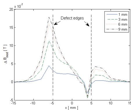
Fig. 4. Numerical simulation results: differential response signals using probe tilting in x-axis, \varphi = 45^\circ tilt
