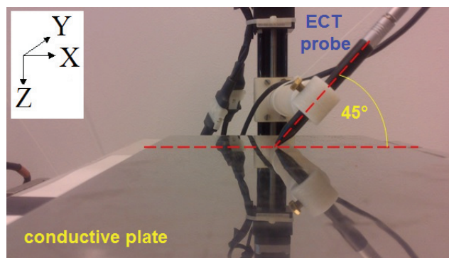
Fig. 10. Configuration of the ECT probe over the conductive specimen with defect
