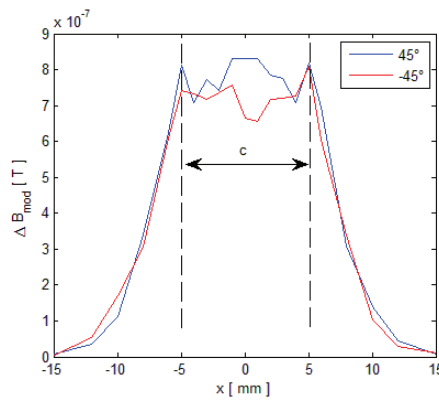
Fig. 9. Numerical simulation results: combination of differential response signals using probe tilting on 3 mm defect
