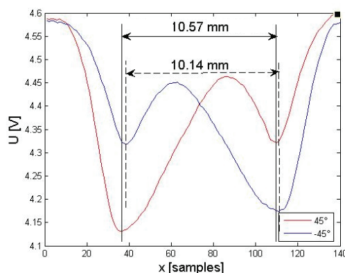
Fig. 12. Imaginary component of response signal – tilted probe scan
