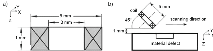
Fig. 2. A) geometry of the ECT probe, b) configuration with tilting positions
