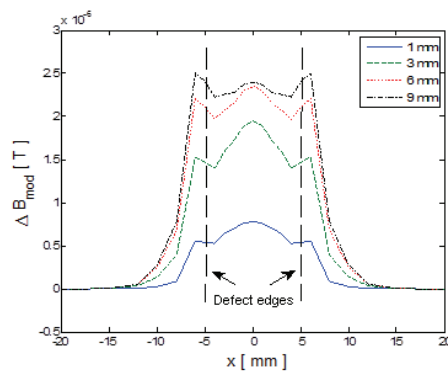
Fig. 3. Numerical simulation results: differential response signals using conventional ECT approach
