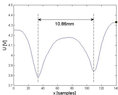
Fig. 11. Imaginary component of response signal – conventional scan
