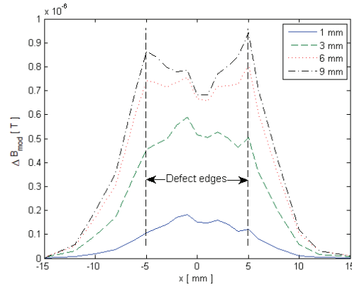
Fig. 8. Numerical simulation results: differential response signals using probe tilting in y-axis, \varphi = -45^\circ tilt
