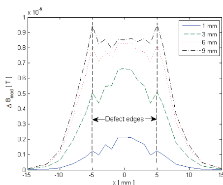
Fig. 7. Numerical simulation results: differential response signals using probe tilting in y-axis, \varphi = 45^\circ tilt
