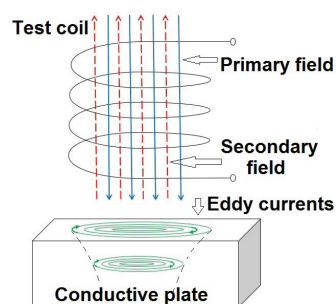
Fig. 1. Principle of the ECT method
