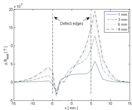
Fig. 5. Numerical simulation results: differential response signals using probe tilting, in x-axis, \varphi = -45^\circ tilt
