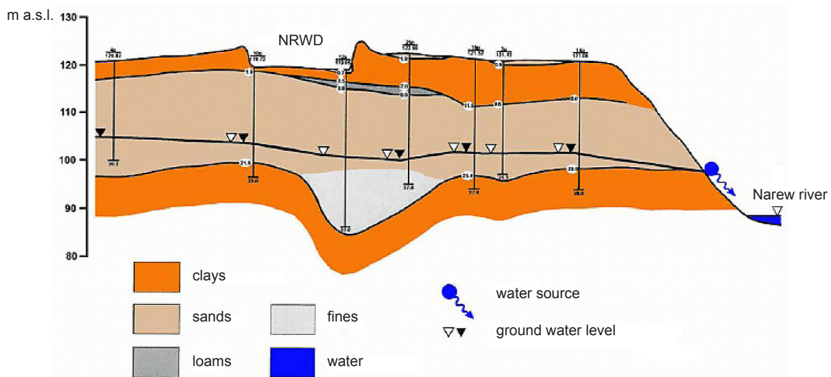
Fig. 2. Hydrogeological system profile of National Radioactive Waste Dump in Róźanie [Madaj 2010]
