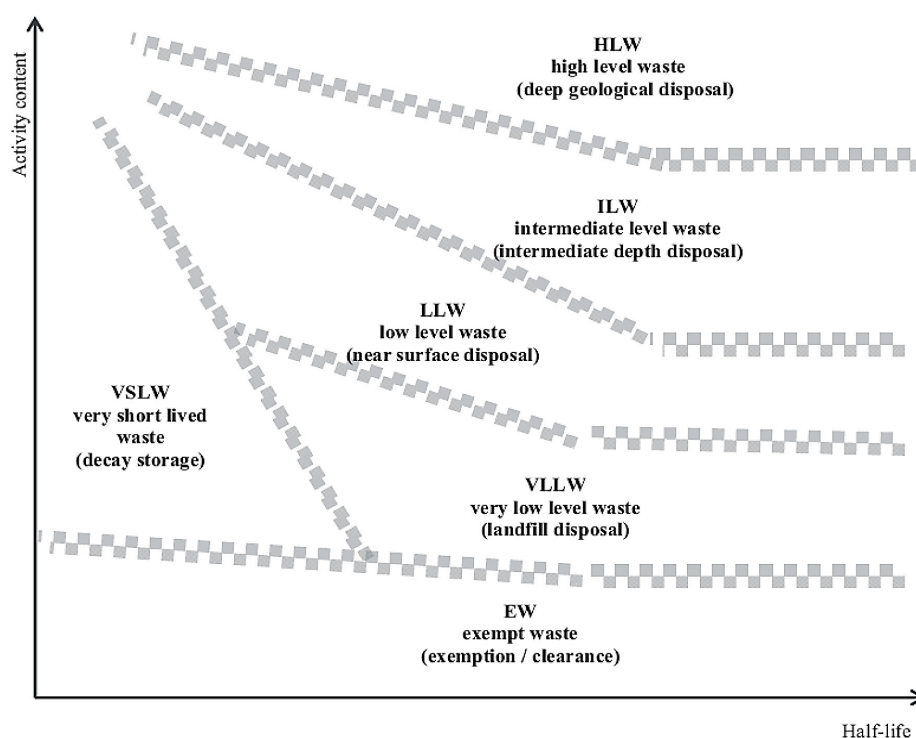
Fig. 1. Classification of solid radioactive waste in terms of their activity [IAEA 2009]
