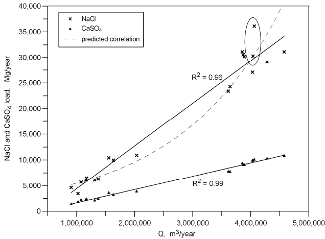
Fig. 4. Chlorides and sodium loads as NaCl and sulphates and calcium as \text{CaSO}_4 captured by the wells barrier near the facility vs. abstracted saline water ( Q )
