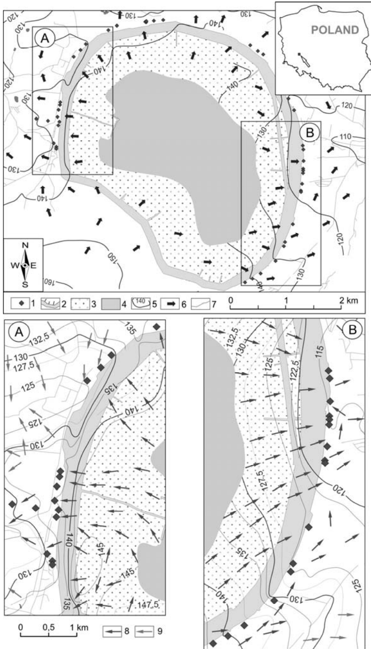
Fig. 1. Żelazny Most tailings disposal site and a wells barrier: 1 – drainage well, 2 – dam, 3 – tailings, 4 – sludge supernatant pond, 5 – contour line of groundwater head, 6 – main directions of groundwater flow in the Quaternary porous aquifer, 7 – water courses, 8 – flow directions of contaminated groundwater in aquifer, 9 – flow directions of fresh groundwater, A, B – fragments of western (A) and eastern (B) part of the disposal site and its foreground
