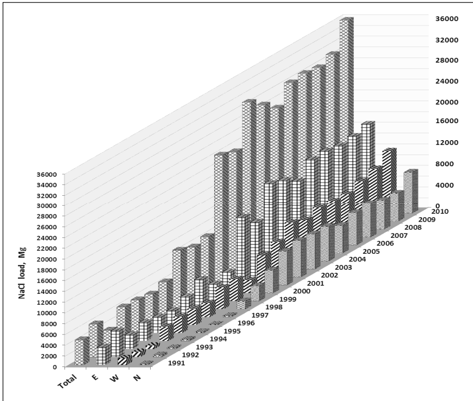
Fig. 5. Time series of NaCl load captured by barrier wells near the facility and along its dams. Total – the whole facility, dams: E – eastern, W – western, N – northern
