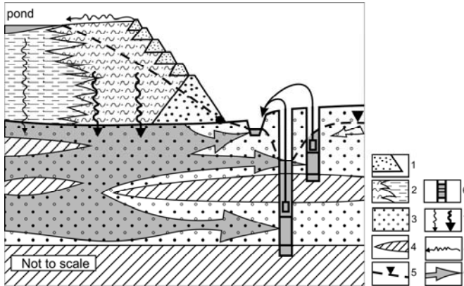
Fig. 2. Model of capturing contaminated groundwater by a drainage wells barrier (after [21], modified): 1 – dam, 2 – tailings, 3 – sandy deposits, 4 – low permeable deposits, 5 – groundwater head, 6 – drainage well, 7 – saline water seepage through tailings, 8 – tailings silting up, 9 – directions of contaminated groundwater flow in aquifer
