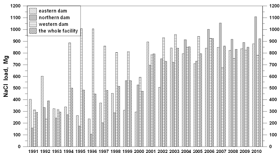
Fig. 6. Time series of NaCl load captured within a year by single well of barrier around the whole facility and in particular barrier parts along the dams
