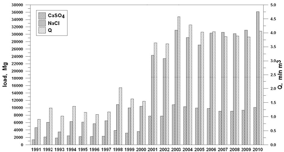
Fig. 3. Time series of chlorides and sodium loads as NaCl and sulphates and calcium as \text{CaSO}_4 captured yearly by the wells barrier near the facility, and abstracted saline water (Q)
